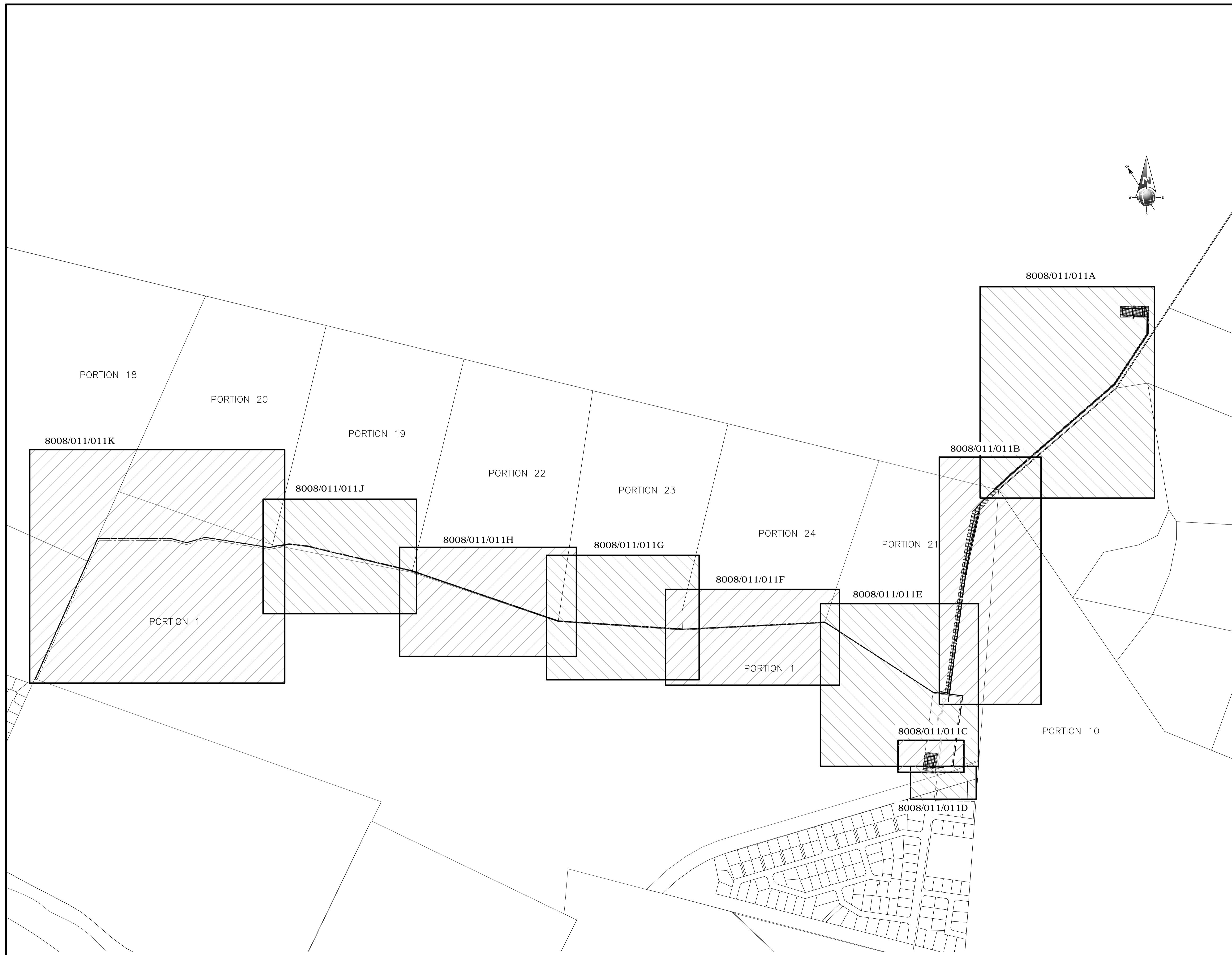
KEY PLAN – SERVITUDE DIAGRAMS SCALE 1:5000
