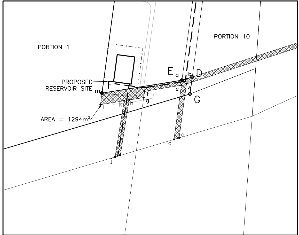
SERVITUDE DIAGRAM NOT TO SCALE
