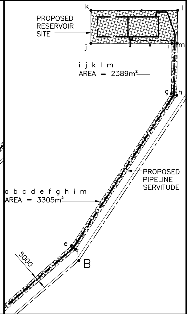
SERVITUDE DIAGRAM NOT TO SCALE
