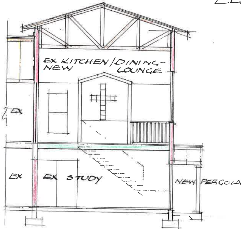
SECTION 'C' (STAIR CASE SUPERIMPOSED)
