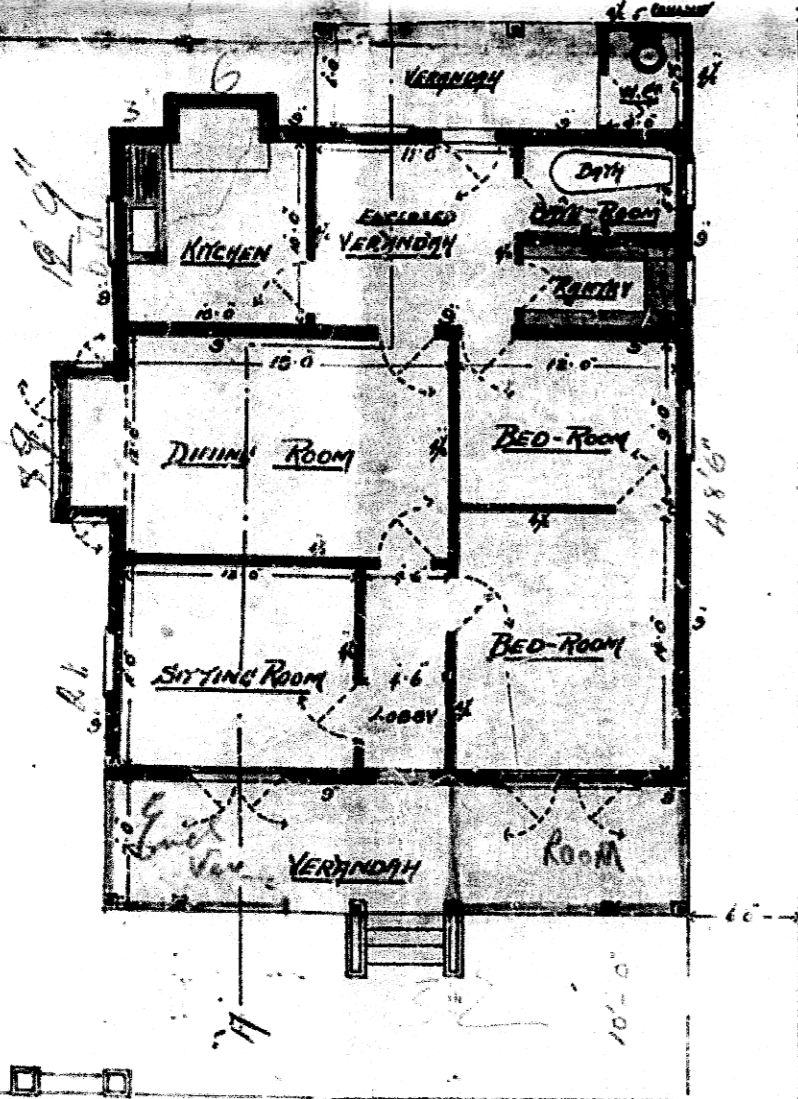
— GROUND PLAN. —
