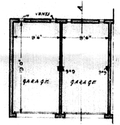
PLAN GARAGE
