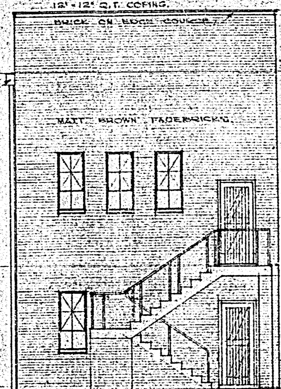
SOUTH-EAST ELEVATION
