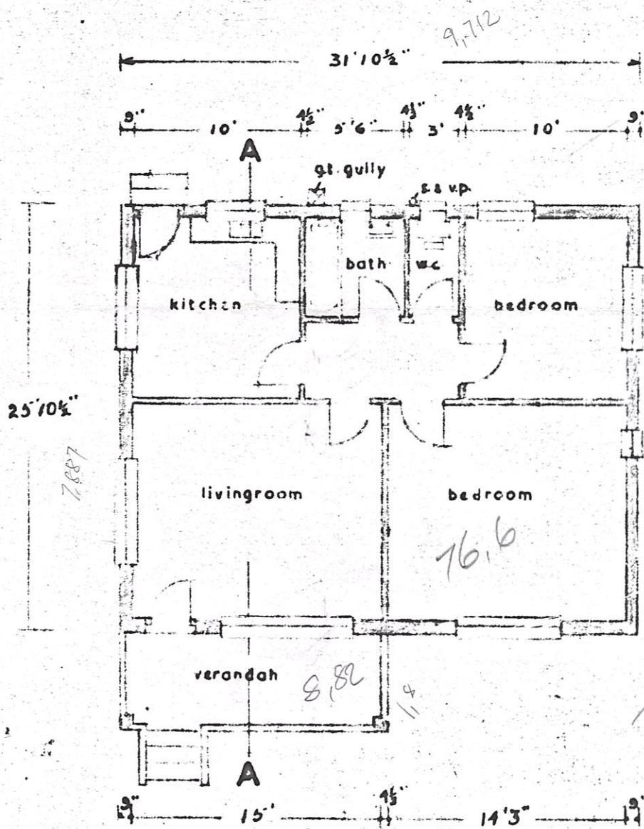
PLAN
