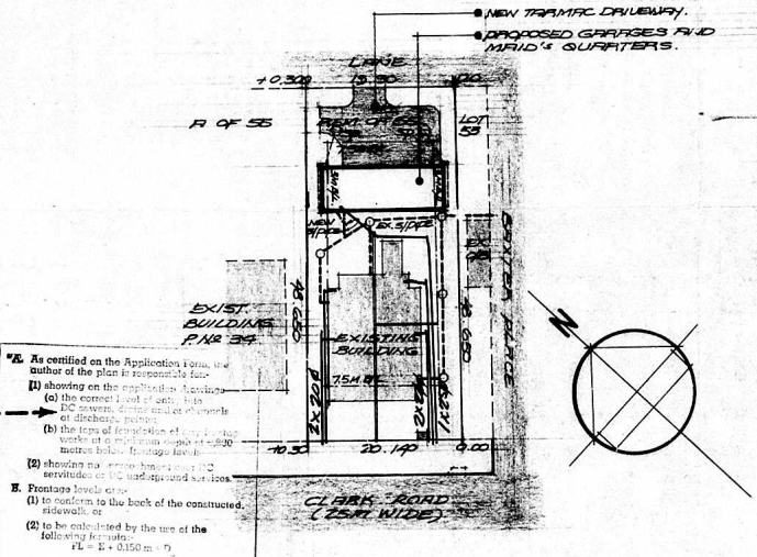
● site plan
