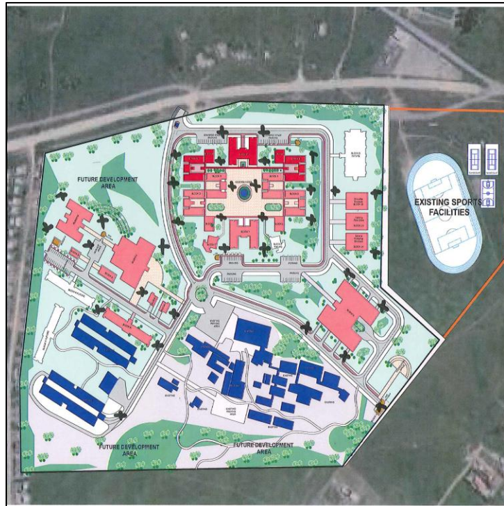
Figure 2: Map showing alternative layout B for the proposed uMzimkhulu FET College
