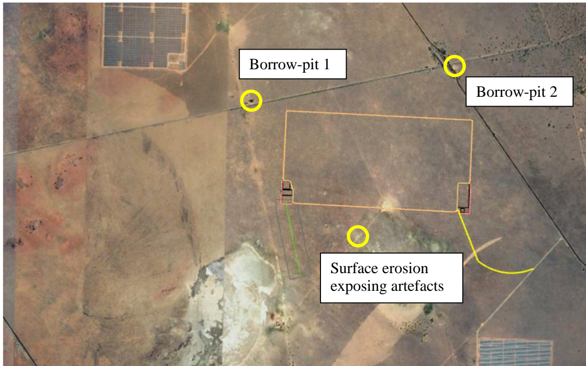
Figure 5. Borrow pits and surface erosion feature (yellow circles) where (in the case of the borrow pits which were recorded in 2018) low density sub-surface Stone Age occurrences were observed and (in the erosion feature, recorded in July 2022) a very small number of the surface artefact finds were noted. The erosion feature is in a pan setting north east of Droogfontein 5 Option A (and south of Droogfontein Option B).
