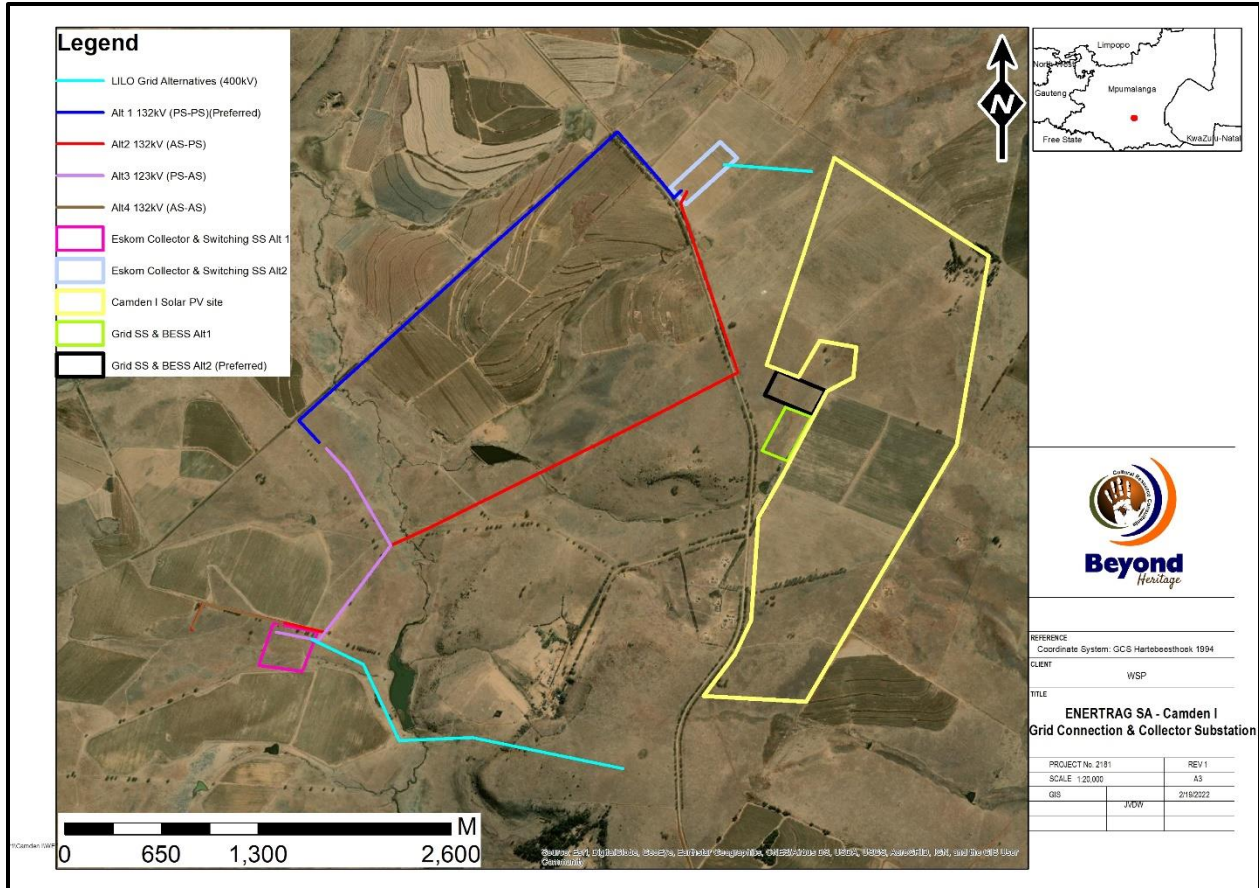
Figure 1.3. Aerial setting of the Project. The boundary of the Camden I Solar Energy Facility, SS & BESS location options and Camden Collector Substation are included to serve as reference points.
