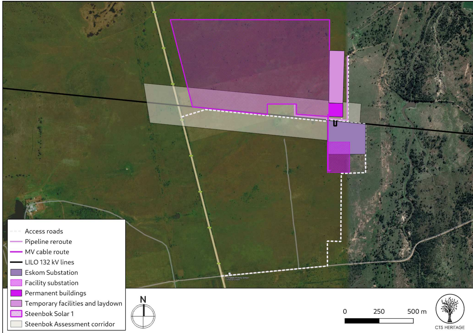
Figure 5: Final Optimised Layout for Steenbok Solar 1 Project
