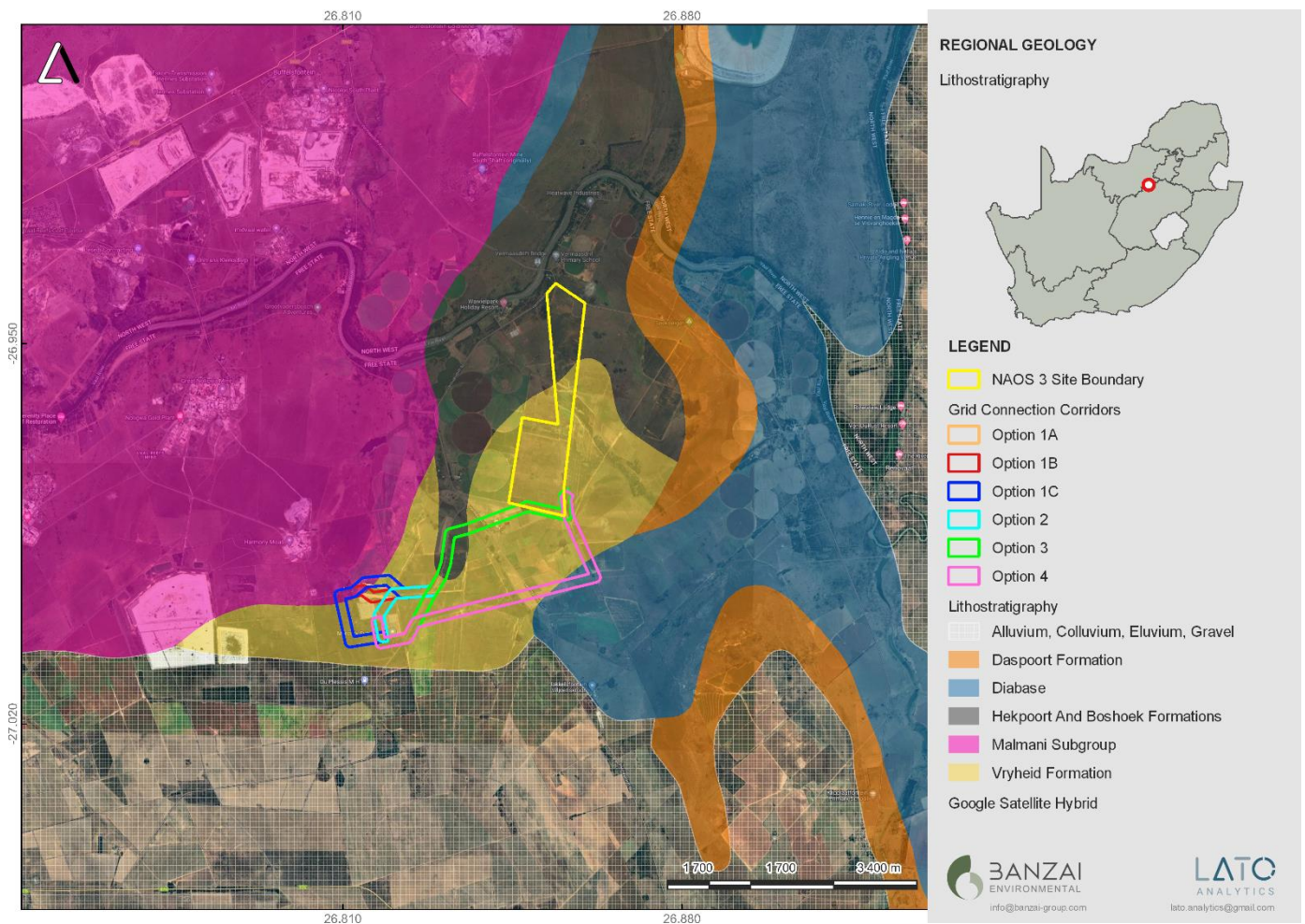
Figure 11: Updated Geology (Council of Geosciences, Pretoria) of the proposed Naos Solar PV Three Project and grid connection near Viljoenskroon in the Free State.
