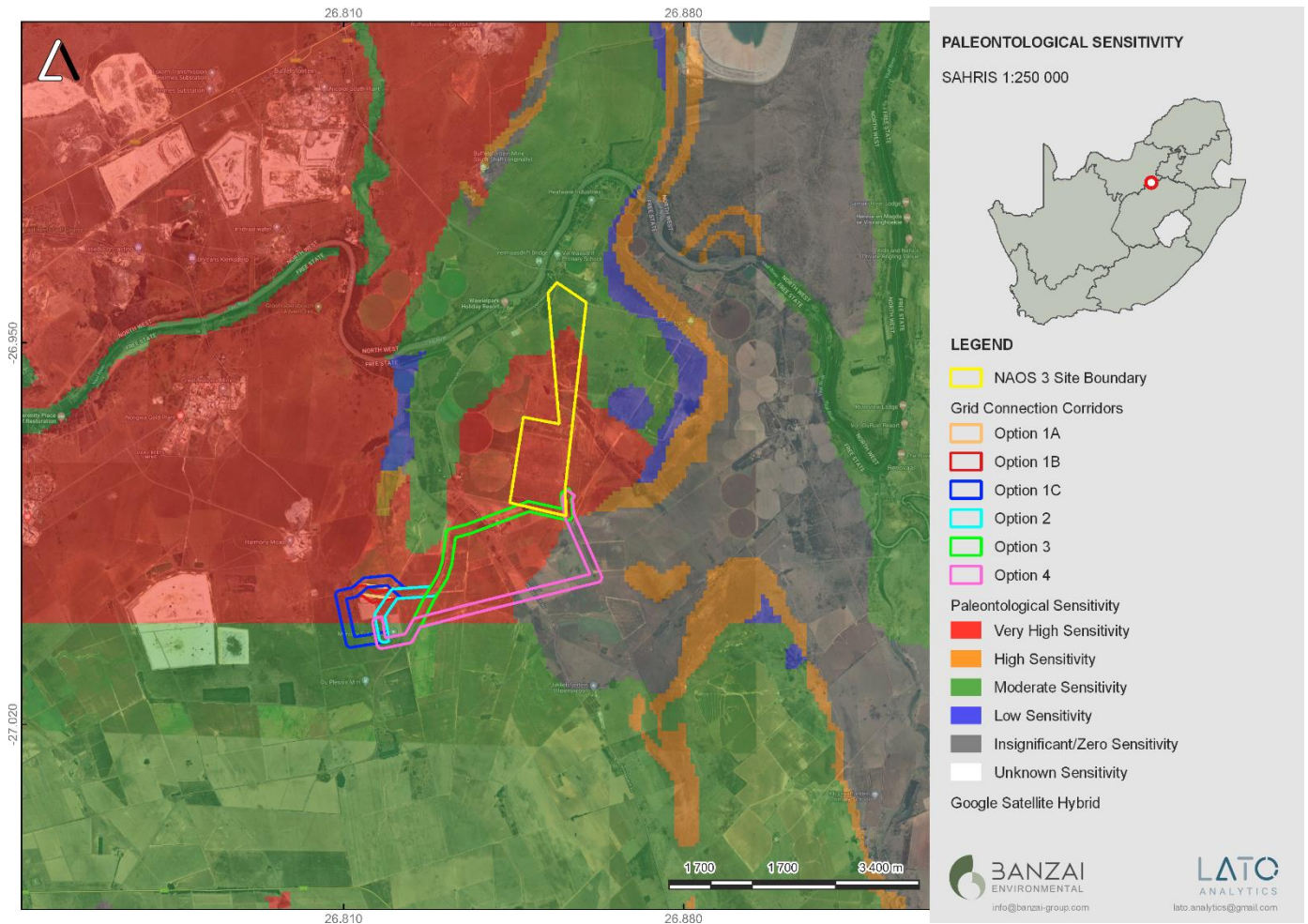
Figure 10: Extract of the 1 in 250 000 SAHRIS PalaeoMap map (Council of Geosciences) indicating the Naos Solar PV Three Project and grid connection alternatives near Viljoenskroon in the Free State.
