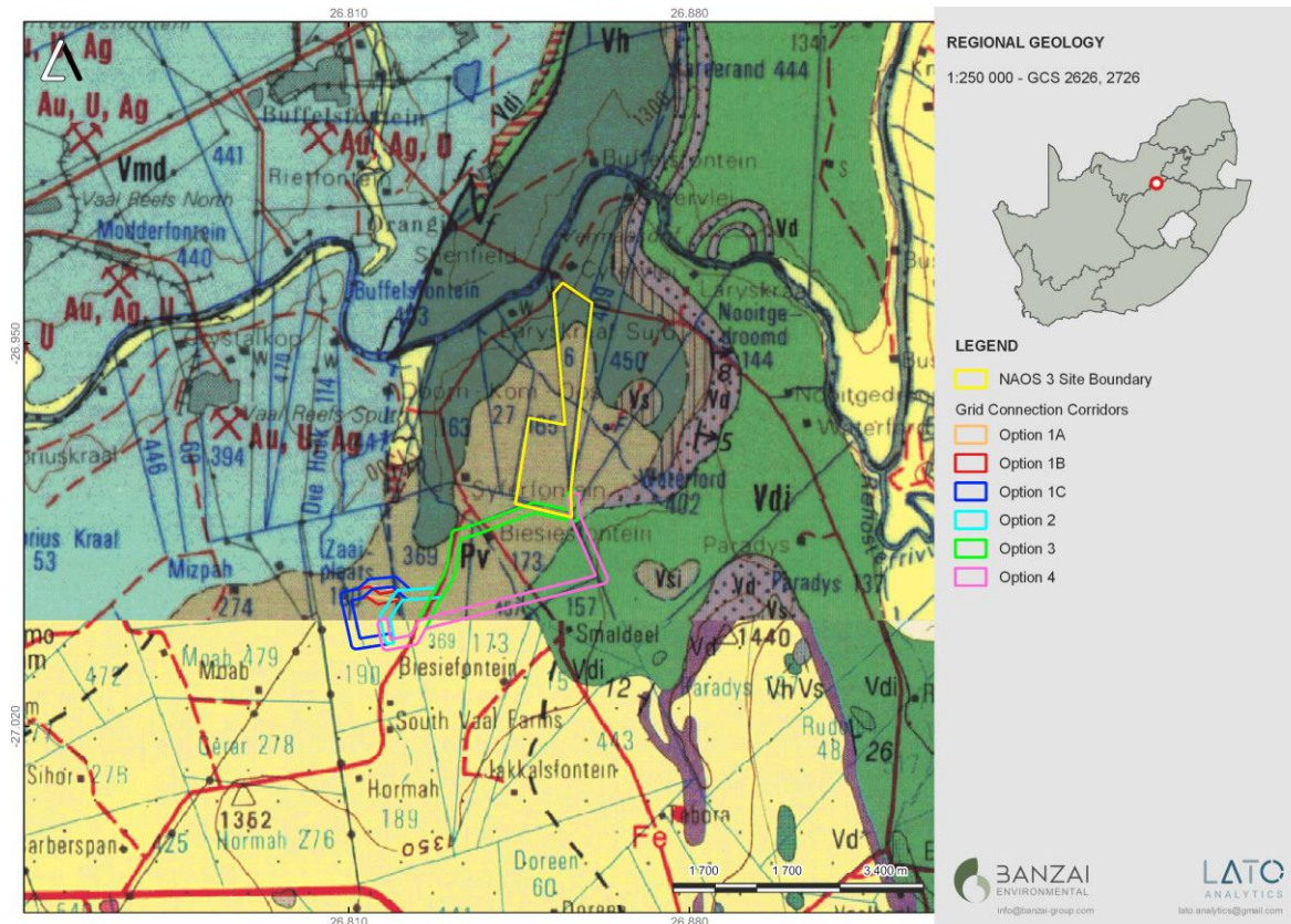
Figure 9: Extract of the 1:250 000 Wes-Rand 2626 (1986) and 2726 Kroonstad (2000) Geological Map (Council for Geosciences, Pretoria) indicating the proposed Naos Solar PV Three Project near Viljoenskroon in the Free State.
