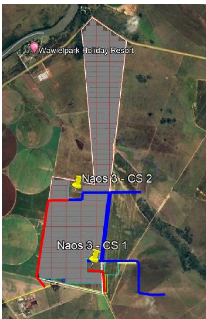
Figure 4: Internal grid connection solution, with two collector substation alternative locations, for Naos Solar PV Project Three (red lines = Naos 2 132kV Eskom power line connecting to the main grid connection corridor for each collector substation alternative, blue lines = Naos 1 & 3 132kV power lines crossing over the Naos Solar PV Project Three).
