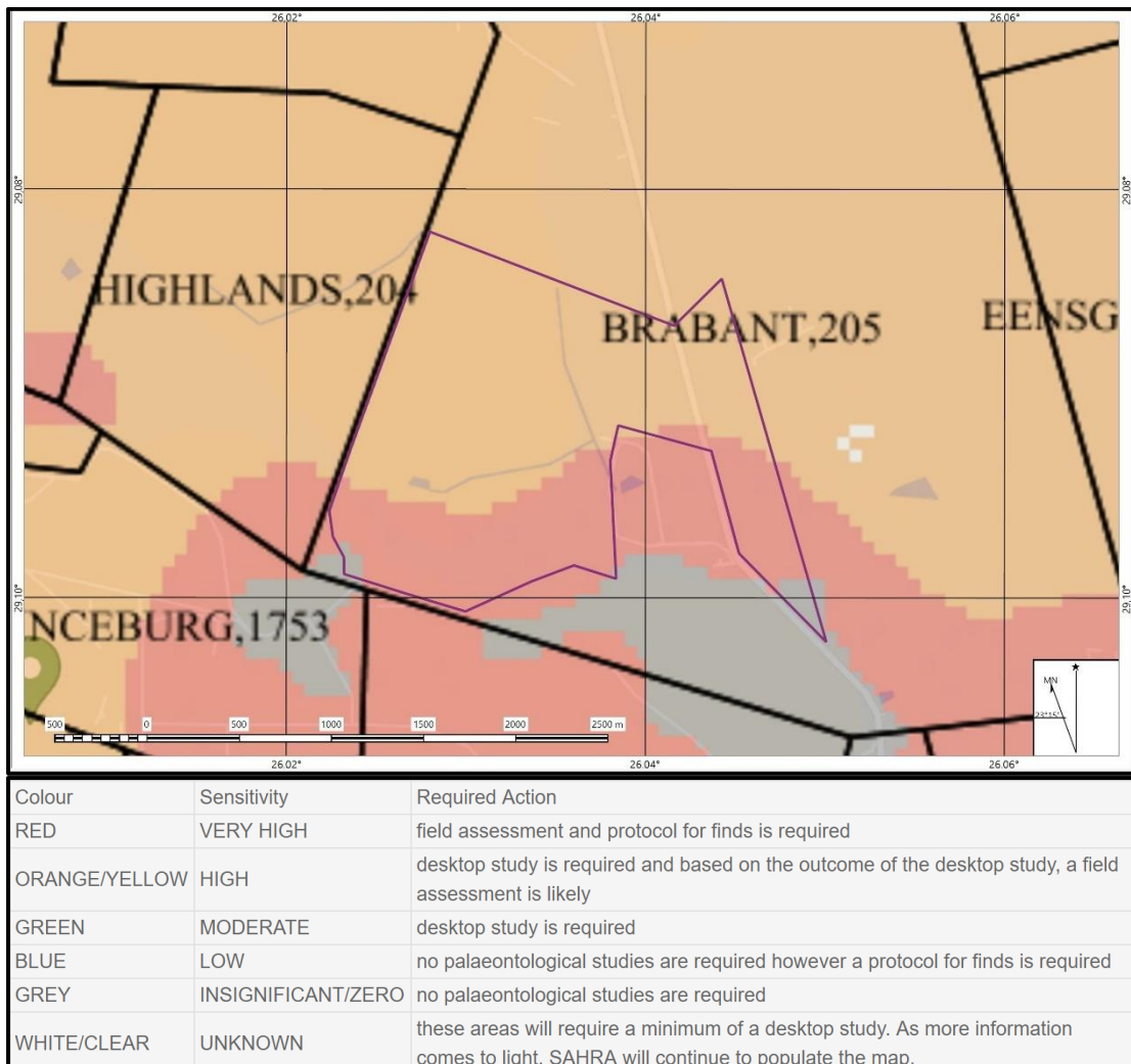
Figure 6. The Palaeontological sensitivity of the project area
