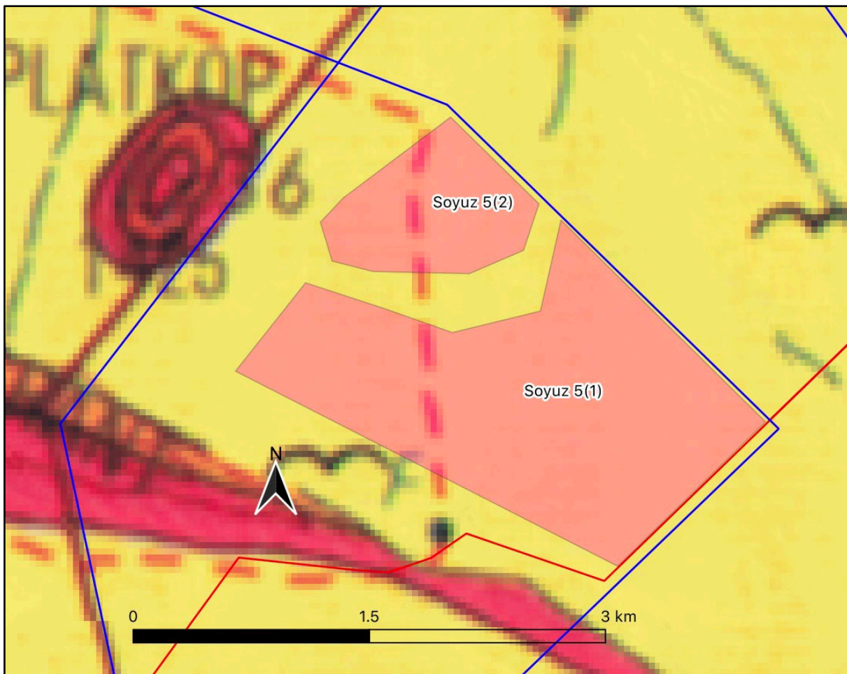
Figure 3: Extract from the 1:250,000 geological chart of the Britstown area showing the location of the Soyuz 5 SPV park on Quaternary sands (yellow) (Source: Geological Survey 1:250 000 map 3022 Britstown).
