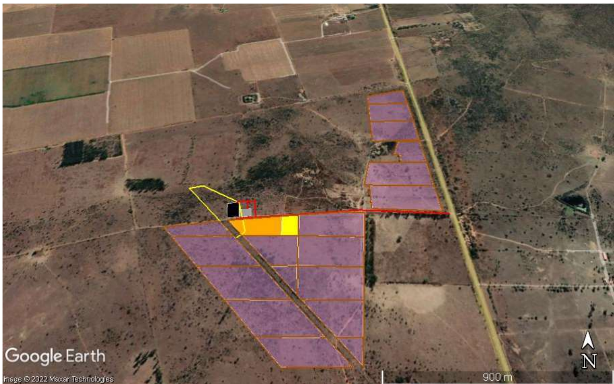
Figure 2: Google Earth Map of the proposed development of the Doornhoek 2 PV Facility with the sections shown by the orange outline. Lilac sections are for the PV collectors, orange and yellow polygons are the amenities, with red lines for the grid connection.
