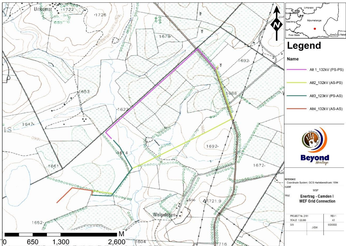
Figure 2: Regional Map of the proposed four alternative routes proposed for the Grid Connection for the Camden I Wind Energy Facility.
