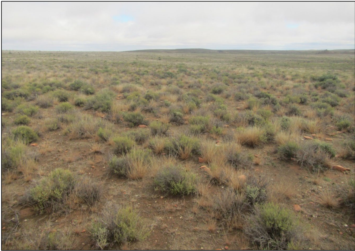
Figure 8: Looking towards the southwest from the north-eastern corner of the WEF site and showing a sandy substrate.
