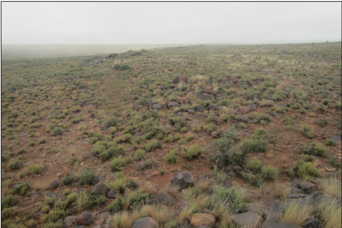
Figure 7: Looking towards the southeast through the northern part of the WEF site showing a dolerite outcrop.
