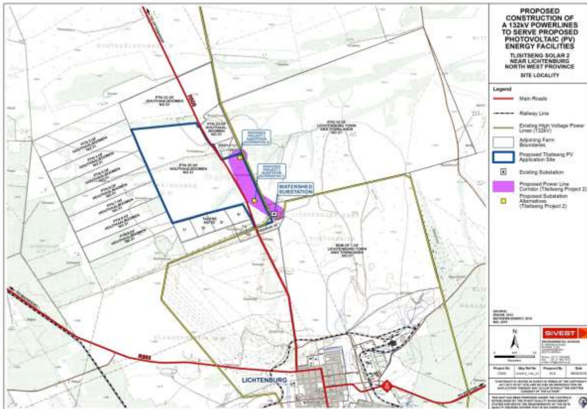
Figure 2 - Tlisitseng Solar 1 – Grid Locality
