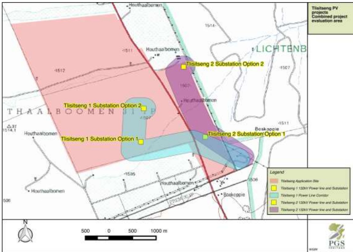
Figure 10 - Combined project options for the Tlisitseng PV facilities
