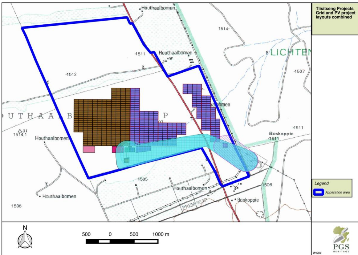
Figure 8 – Total layout for the Tlitseng Solar Projects
