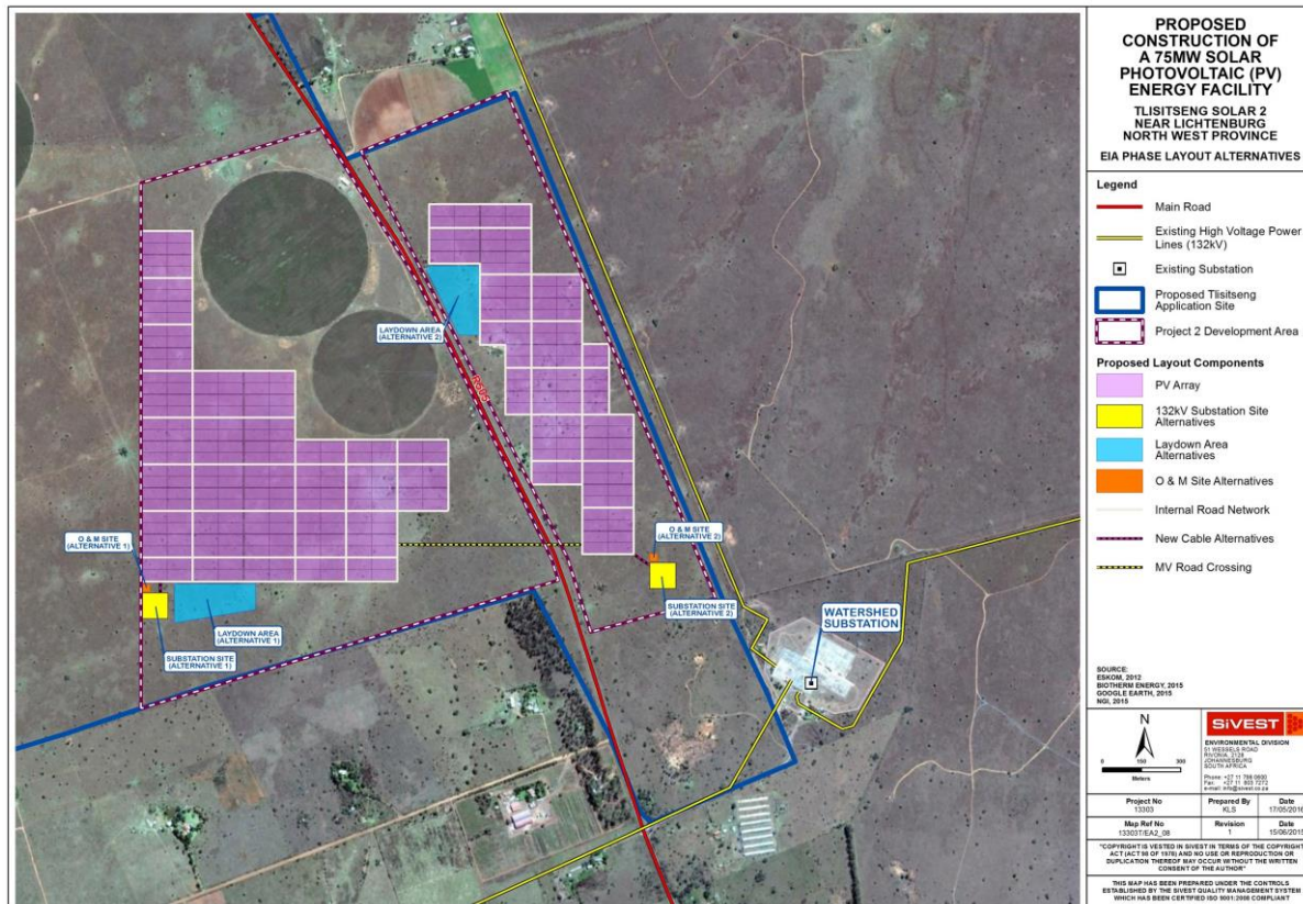
Figure 3 - Tlisitseng PV2 Layout
