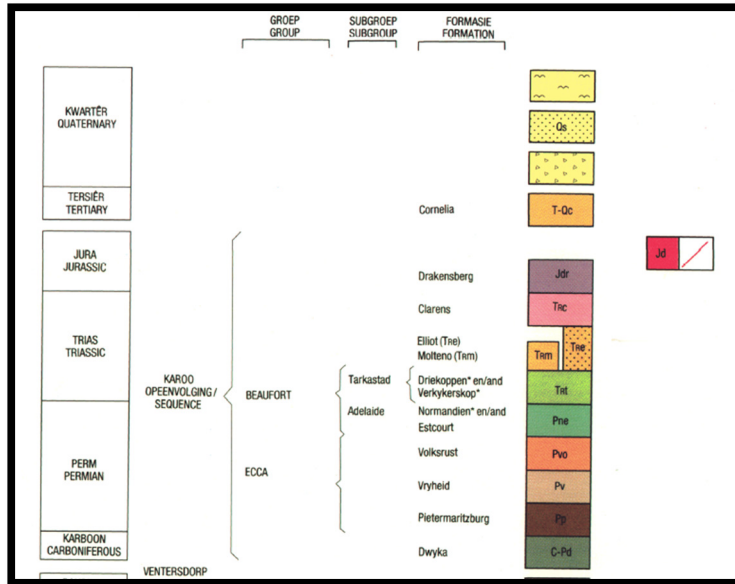
Figure 4: Lithostratigraphic column to show the Eccca Group within the Karoo Supergroup (Muntingh 1992).
