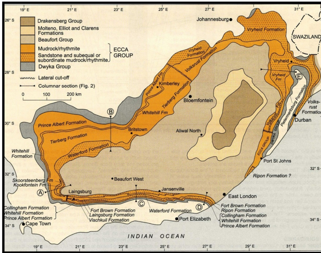
Map 1: Map to show extent of the Ecca Group, more specifically the Vryheid Formation and the Volksrust Formation (Johnson 2009).
