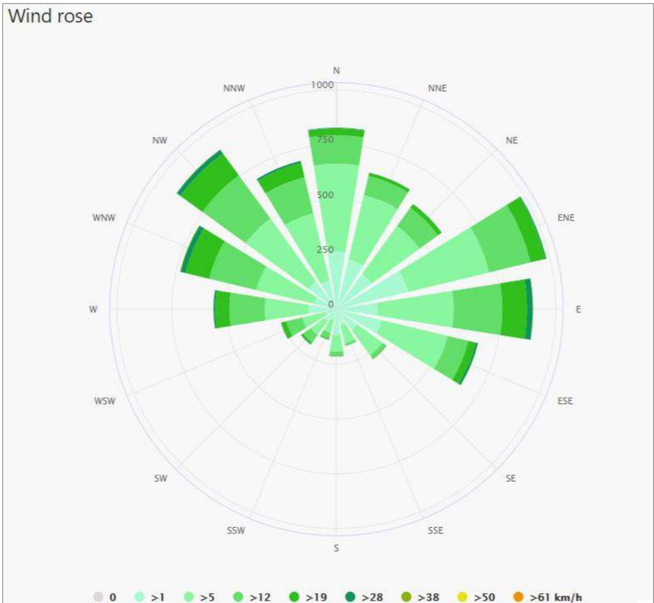
Figure 9: NEMS 30 km simulation model wind rose for the proposed Blesboklaagte project area for the period 1985 to current.
