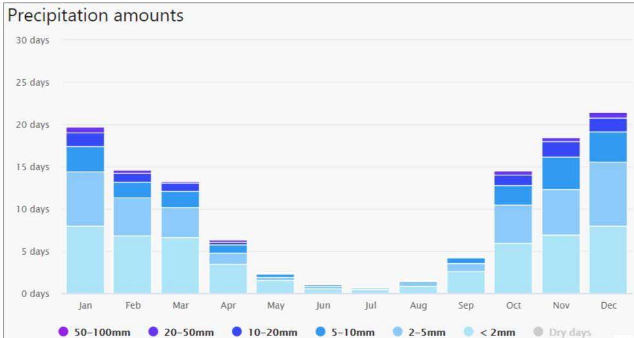
Figure 12: Day count of total daily precipitation per month for the proposed Blesboklaagte project area for the period 1985 – current.
