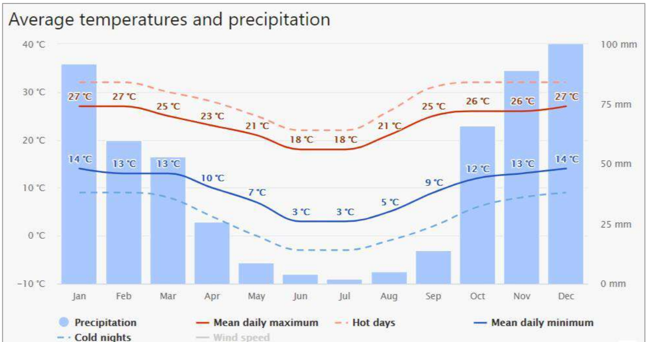
Figure 10: Temp and precipitation simulation results from the NEMS model for the Blesboklaagte project area (1985 - current).
