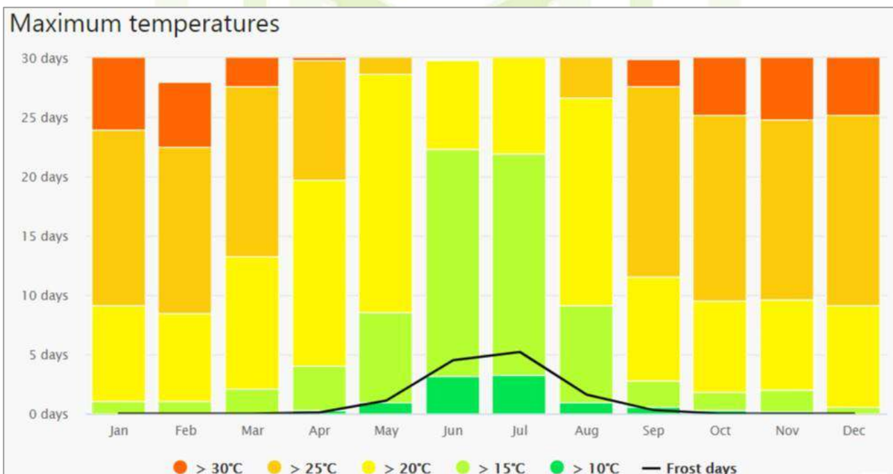
Figure 11: Maximum temperatures as simulated from the NEMS 30 km model for the proposed Blesboklaagte project area (1985 – current).
