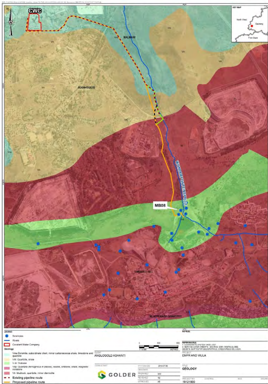
Figure 3: The geology of the development area (Golder from Keyser 1986).
