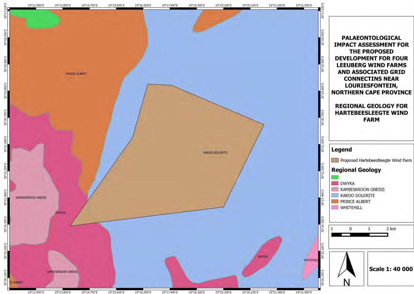
Figure 4: The surface geology of the proposed Hartebeesleegte Wind Farm near Loeriesfontein in the Northern Cape Province. The development footprint is mostly underlain by Karoo Dolerite and a small area in the south west is underlain by the lowermost unit of the Karoo Supergroup, namely the Dwyrka Group.
