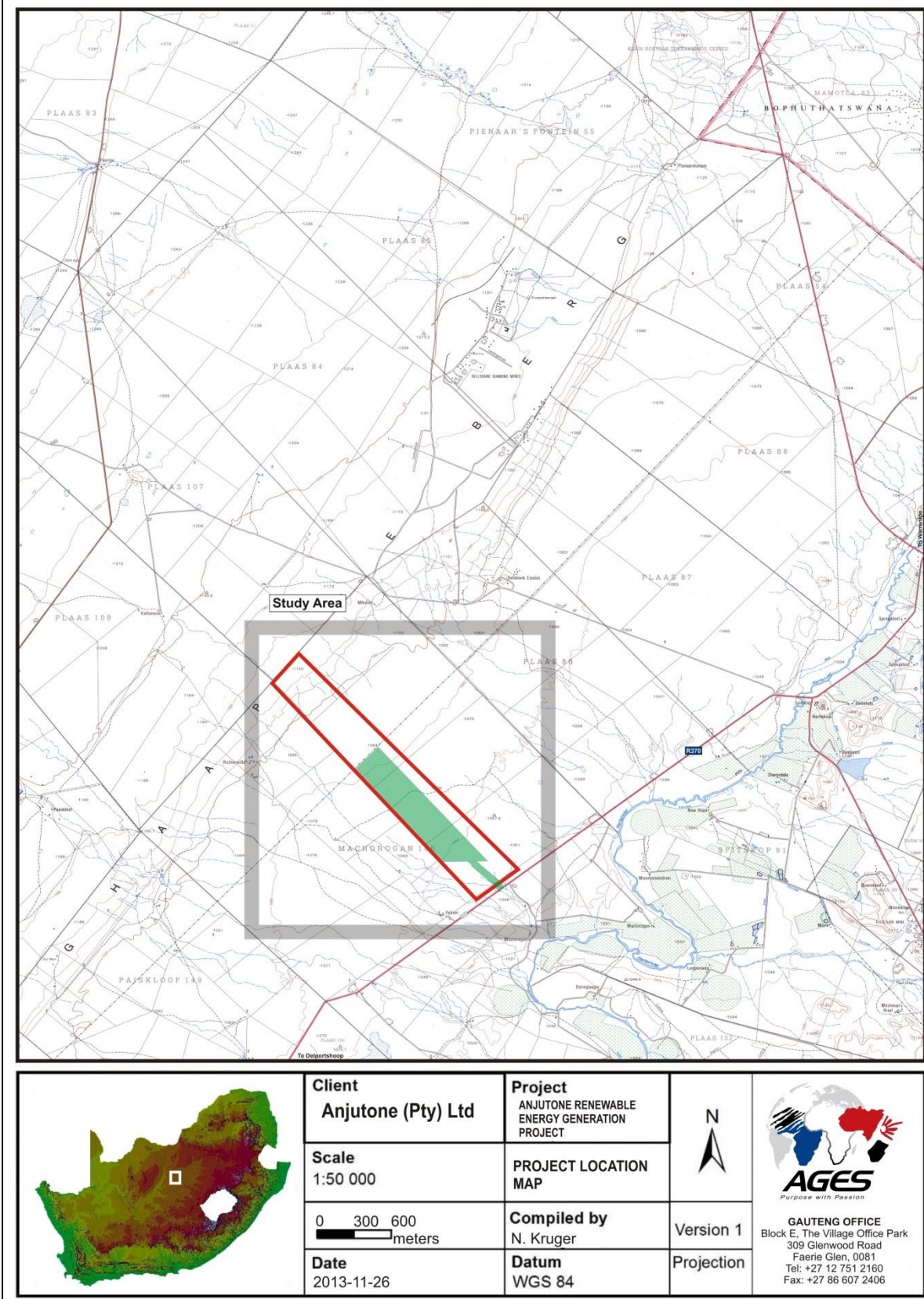
Figure 2-1: 1:50 000 Map representation of the location of the Anjutone Photovoltaic Power Plant and Power Line Development location (2824AB). The farm Machorogan is indicated in red outline and the proposed project footprint in shaded green.
