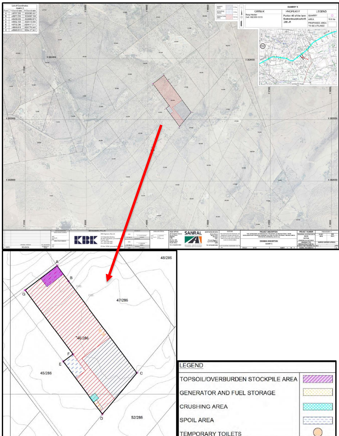
Figure 2. Layout of the proposed quarry (Map supplied by GA Environment)
