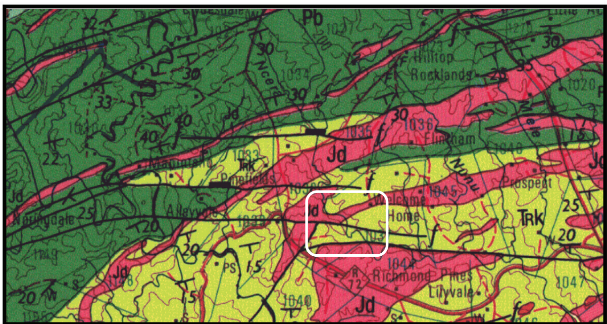
Figure 4: The geology of the development area.
