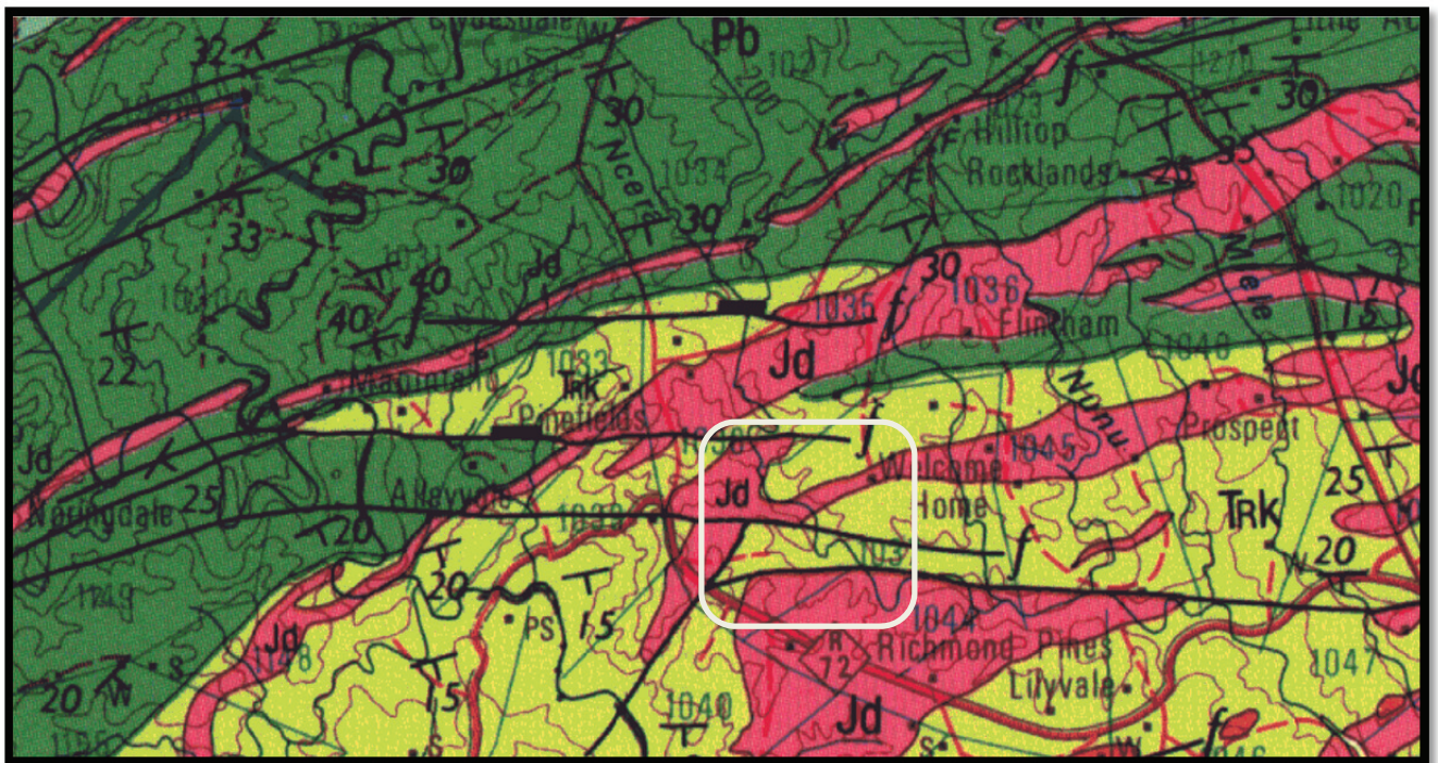
Figure 4: Geology of the development area (Roby and Johnson 1996) (1h).
