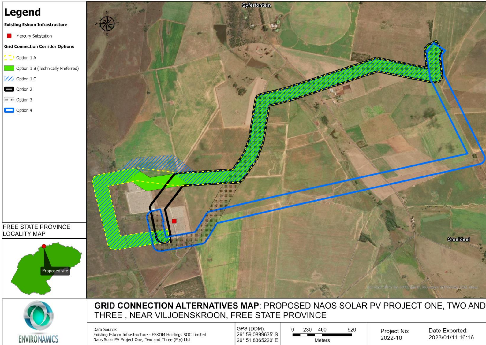
Figure 13: Six grid connection corridor alternatives proposed for the three Naos PV projects.
