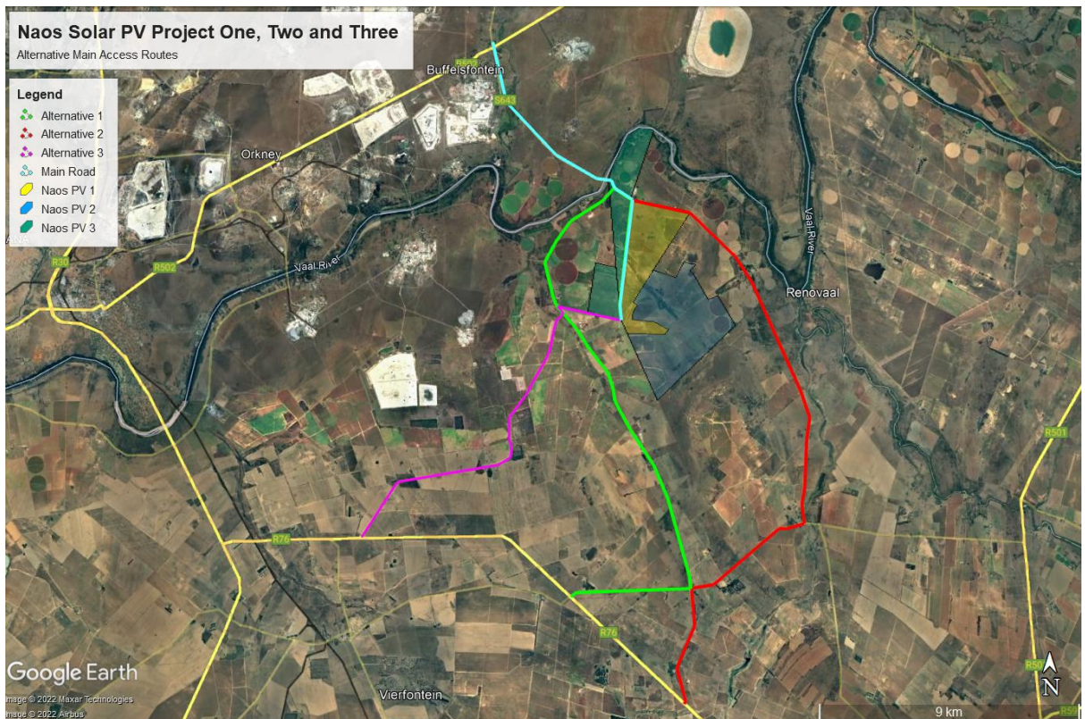
Figure 14: Main access route alternatives proposed for the three Naos PV projects.
