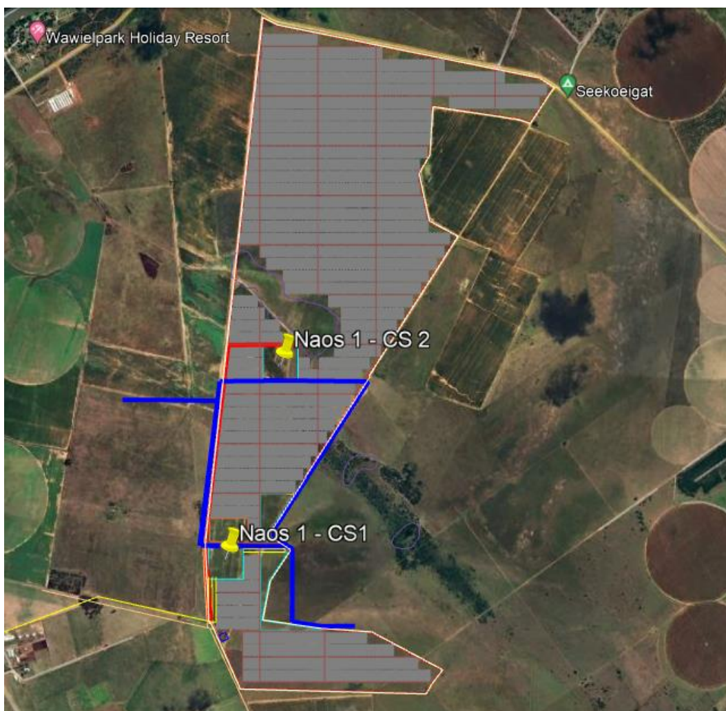
Figure 2: Internal grid connection solution, with two collector substation alternative locations, for Naos Solar PV Project One (red lines = Naos 1 132kV Eskom power line connecting to the main grid connection corridor for each collector substation alternative, blue lines = Naos 2 & 3 132kV power lines crossing over the Naos Solar PV Project One)
