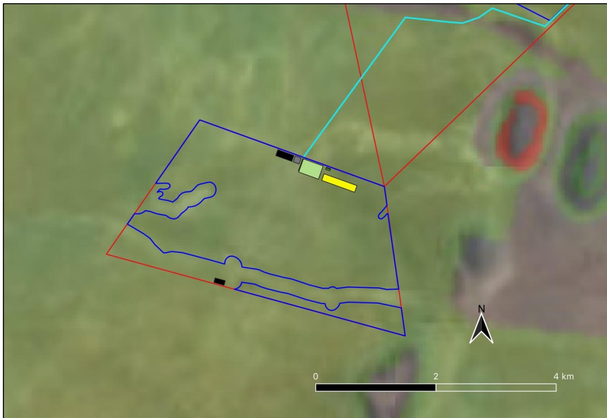
Figure 9: Palaeontological sensitivity indicated on the SAHRIS palaeo-sensitivity map for the Soyuz 1 SPV park. Red shading = very high sensitivity, orange = high, green = moderate, grey = zero (Source: : https://sahris.sahra.org.za/map/palaeo ).
