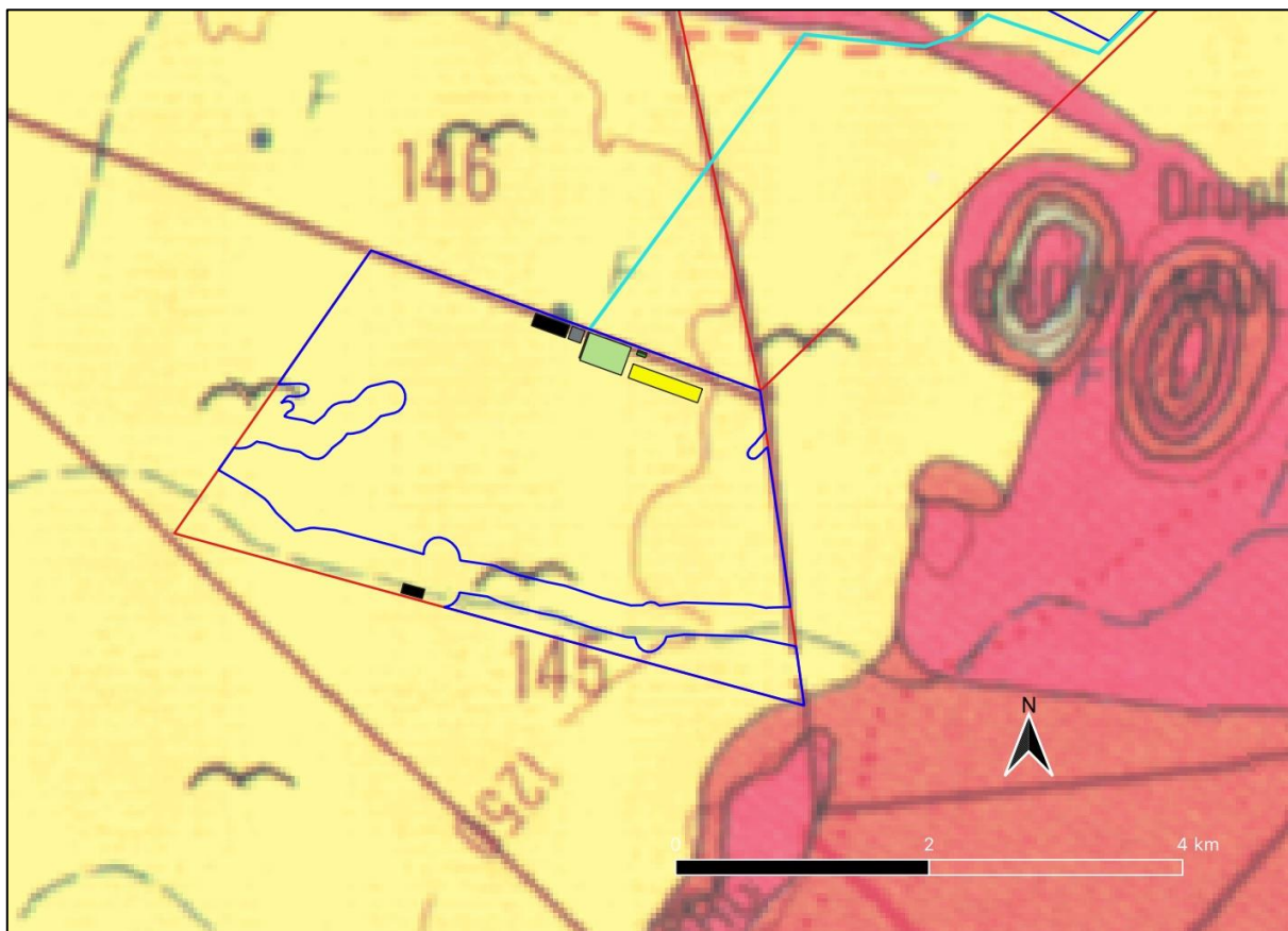
Figure 8: Geological map of the area around the Soyuz 1 SPV Park (blue polygons). Abbreviations of the rock types are explained in Table 2. (Source: 1: 250 000 map 3022 Britstown, Geological Survey).
