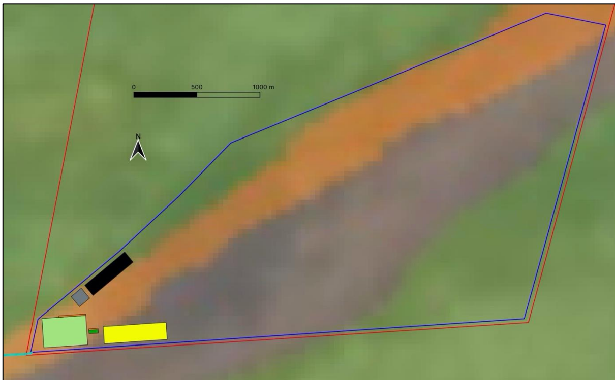
Figure 9: Palaeontological sensitivity indicated on the SAHRIS palaeo-sensitivity map for the Soyuz 6 SPV park. Orange shading = high, green = moderate, grey = zero (Source: https://sahris.sahra.org.za/map/palaeo ).
