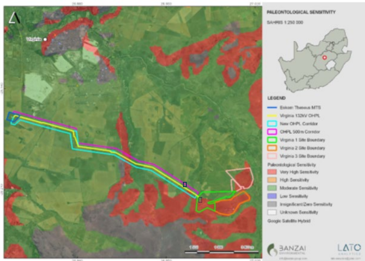
Figure 3: Extract of the SAHRIS Palaeomap (Council of Geosciences, Pretoria) indicating the Virginia 1, Virginia 2, Virginia, 3 and power line corridor. The Virginia 3 PV Solar Park is indicated in peach.
