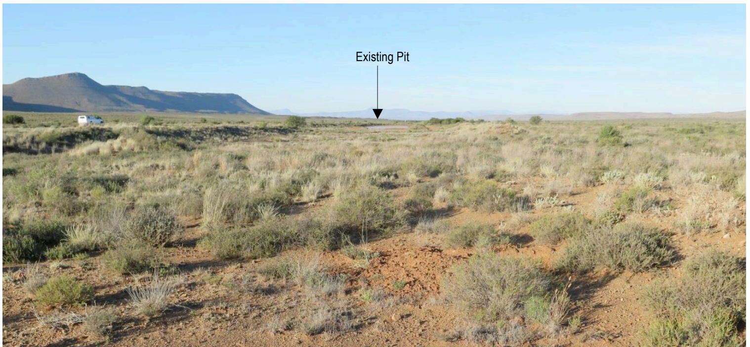
Figure 2: View towards the east showing the gravels in the exposed patches (Tusenius 2015: 7)
