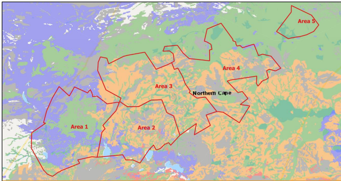
Figure 9: Extract of the 1: 250 000 SAHRIS Palaeosensitivity Map (Council of Geosciences). Approximate location of the proposed five prospecting application areas is indicated in red. Area 3 = Wit Puts Prospecting Application area.
