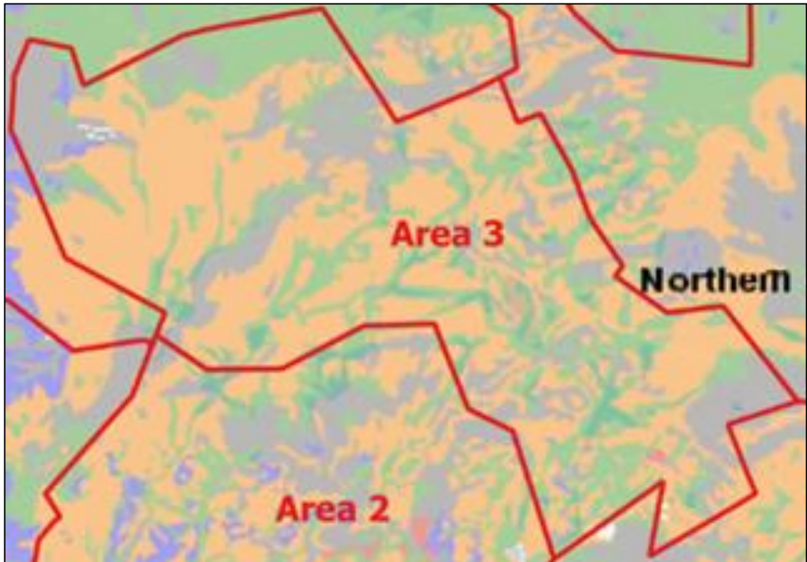
Figure 11: The SAHRIS Palaeosensitivity map indicates that the Wit Puts application area is underlain by geological formations rated as having varying palaeontological sensitivity, from white/grey (Insignificant), to Green (Moderate) and Yellow (High) with some Red (Very High) and some Blue (Low).
