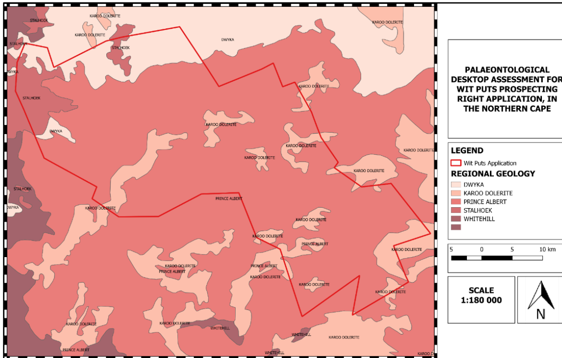
Figure 8: Approximate location and surface geology of the proposed Wit Puts Prospecting area in the Northern Cape 1 . Map drawn by QGIS Desktop 2.18.28
