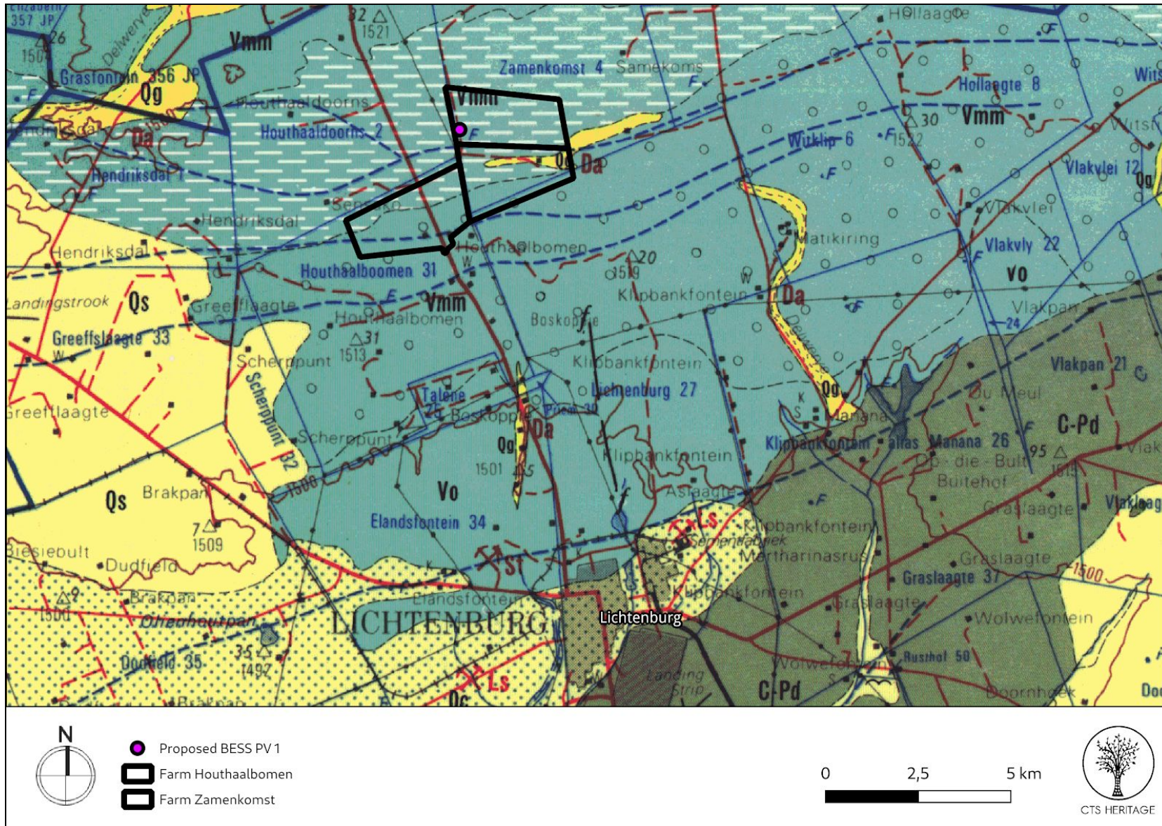
Figure 4b. Geology Map. Extract from the CGS 2626 West Rand Map indicating that the development area for the Lichtenburg 1 PV Facility as well as the development area for the BESS is underlain by sediments of the Monte Christo Formation assigned to the Chuniespoort group, within the Malmani Subgroup (Vmm).
