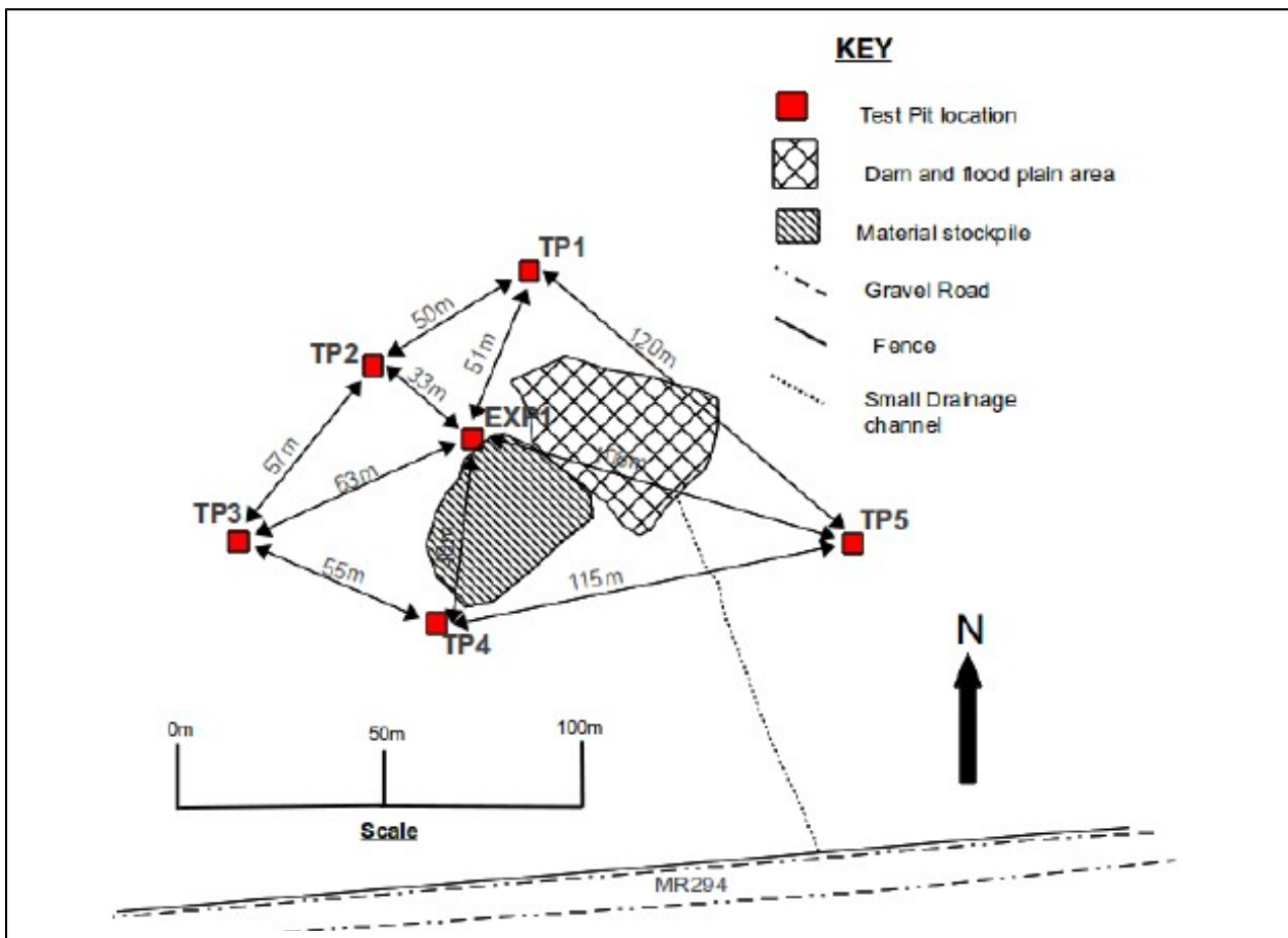
Figure 6: Proposed material to be obtained from the development of a new borrow pit (July 2011)
