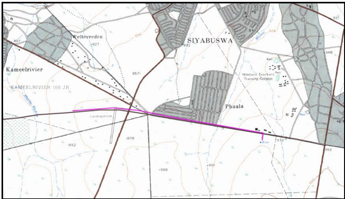
Fig. 2. Location of the study area (outlined in green) (Map 2528BB, 2529AA: Government Printer).
