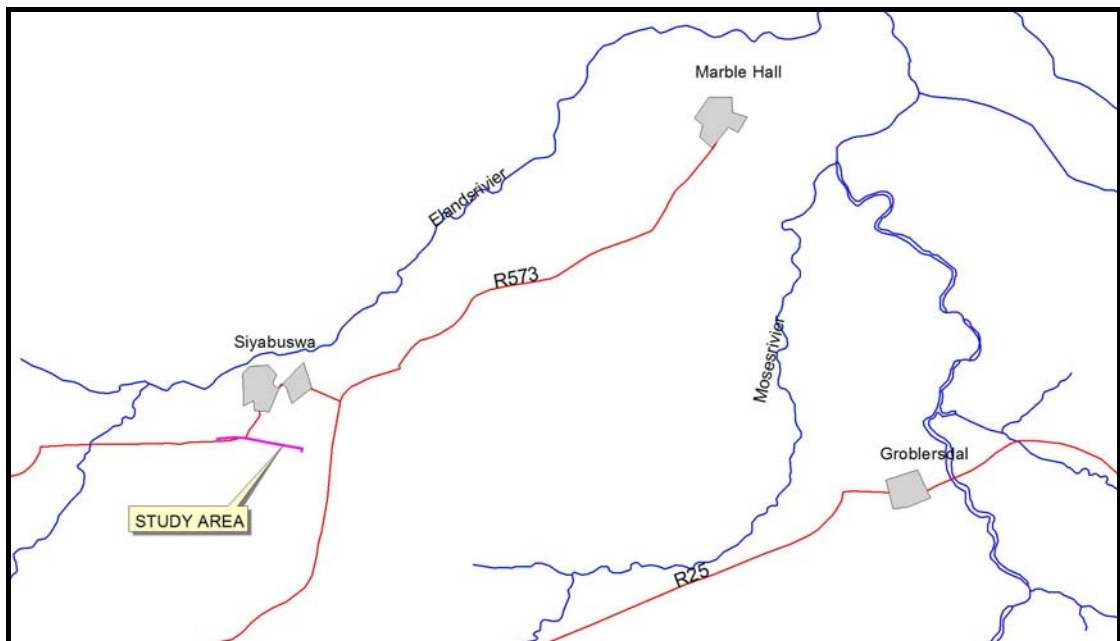
Fig. 1. Location of the study area (outlined in purple) in regional context (Map: Government Printer).
