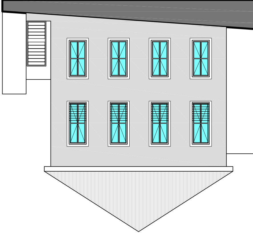
SOUTH ELEVATION 800mm wide openings
