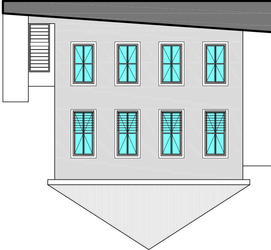
SOUTH ELEVATION 900mm wide openings
