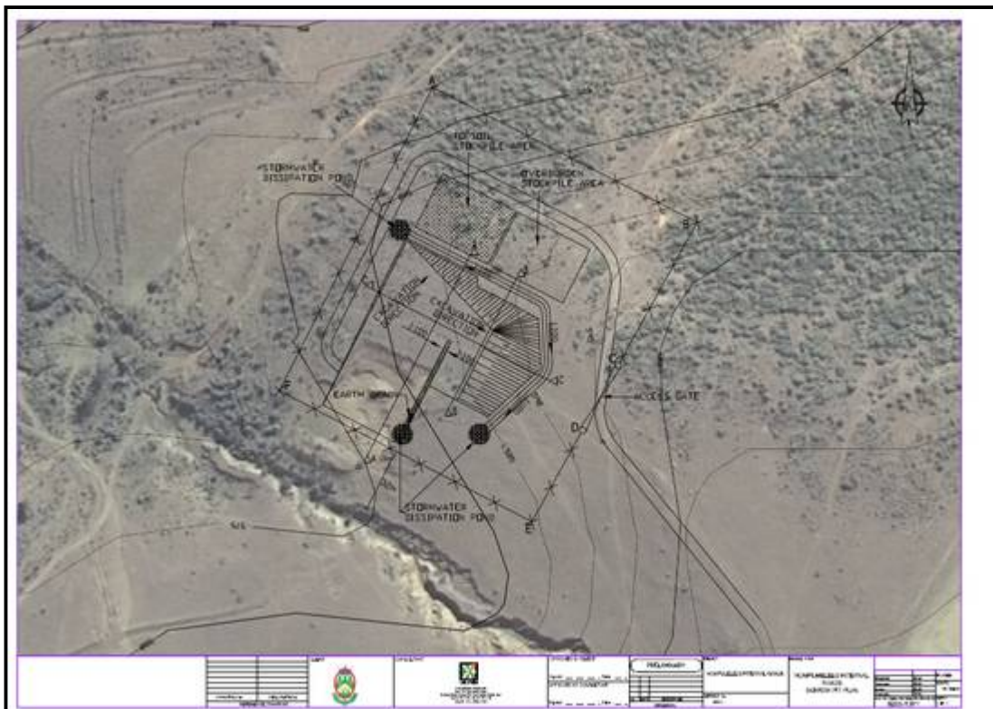
Figure 4: The Nompumelelo Borrow Pit – aerial layout (courtesy Vela VKE Consulting Engineers)
