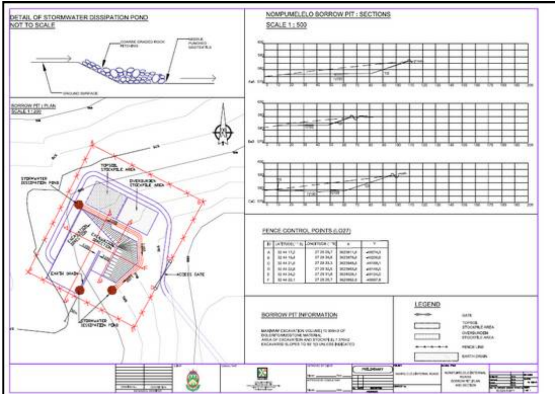
Figure 3: The Nompumelelo Borrow Pit – technical details (courtesy Vela VKE Consulting Engineers)
