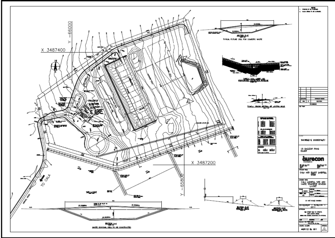
Figure 2: Proposed development layout of the Cala Landfill study site (courtesy Terreco & Aurecon)
