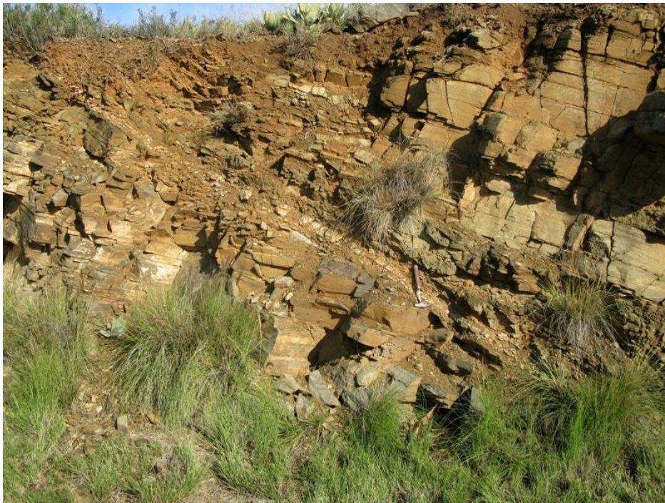
Plate 9-9: East-facing roadcut along the N10 south of Cookhouse showing package of tabular-bedded, horizontally-laminated channel sandstones cut by N-dipping reverse fault that is associated with quartz mineralization and brecciation (above hammer) (Loc. 353) (Hammer = 30cm).
