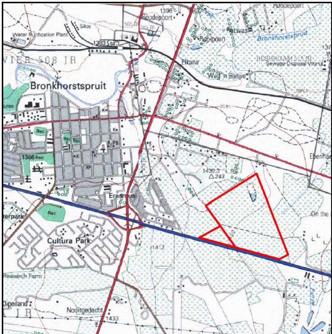
Fig. 1 Location of the study area: Portion 100 is the small triangle on the left (Map 2528DC, 2528DD: Government Printer, Pretoria).
