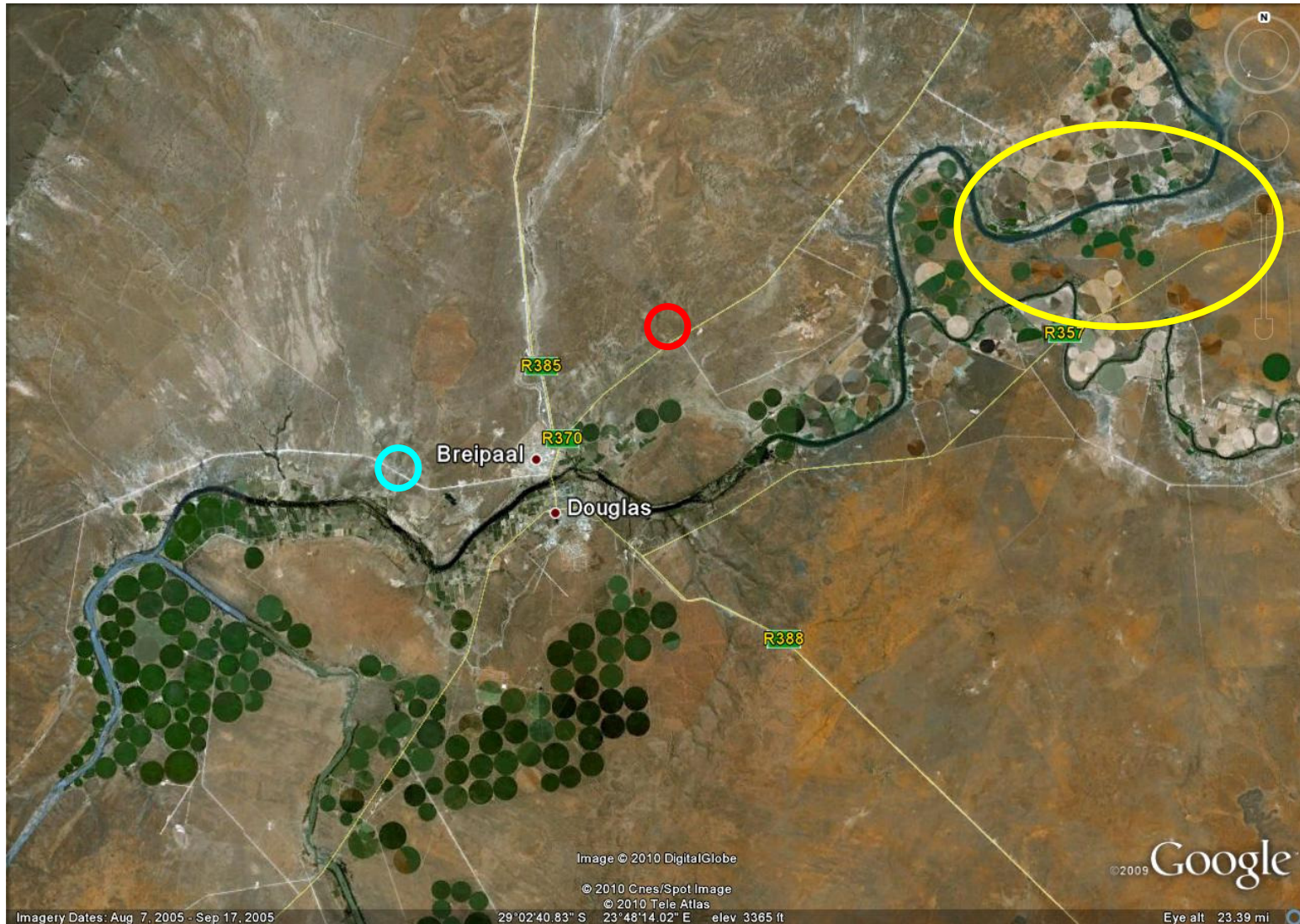
Fig. 1. Google Earth ® satellite image showing the location (red circle) of the proposed photovoltaic power station at the Herbert Substation, north of the Vaal River and c. 7 km northeast of Douglas, Northern Cape Province. The Stratotype C section of the Mbizane Formation (Dwyka Group) is indicated by the blue circle. Key fossil sites within the Prince Albert Formation are found along the Vaal River c. 10 km to the east of Herbert Substation within the area indicated by the yellow ellipse (See also map Fig. 5 below).
