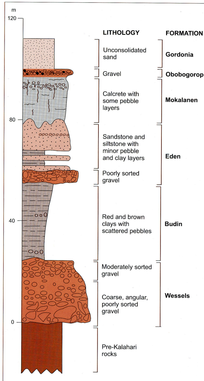
Fig. 3. Stratigraphy of the Kalahari Group (From Partridge et al. , 2006). Aeolian sands of the Gordonia Formation as well as calcretes possibly equivalent to the Mokalanen Formation are represented in the study area.
