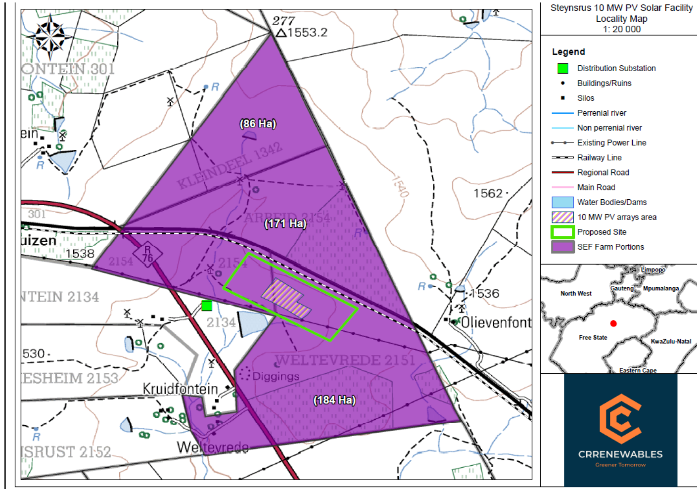
Locality Map of the Proposed Steynsrus 10MW PV Solar Facility and Storage
