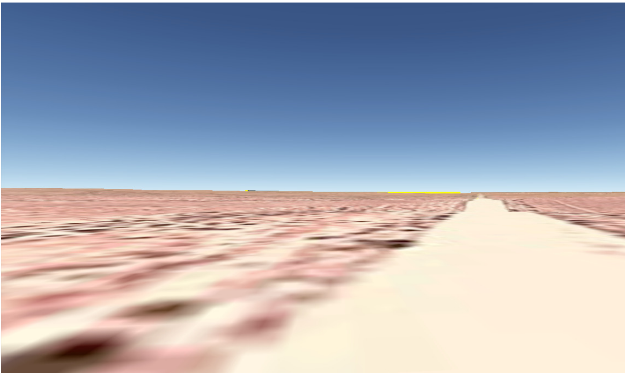
Figure 26: Google Earth 3D perspective view from similar northbound location (yellow = Bravo PV, Green = Substation, Blue = Power Line).
