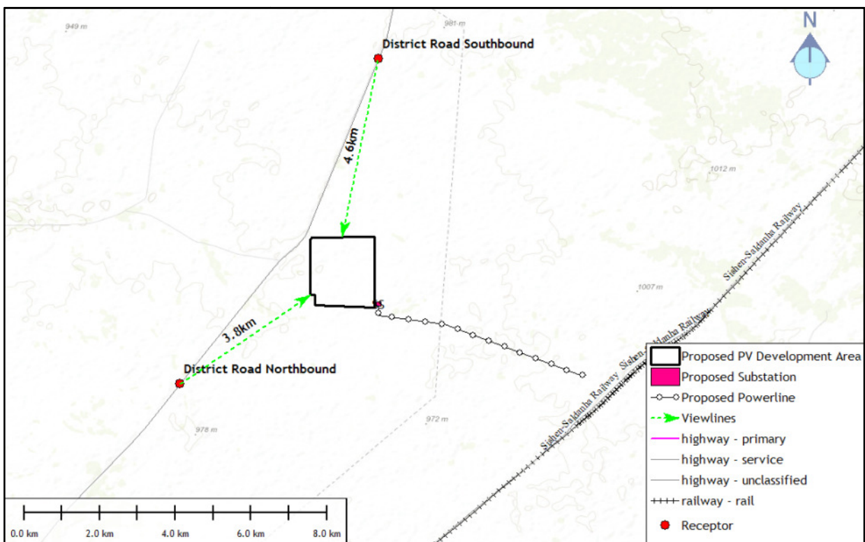
Figure 22: Map depicting the main receptor locations associated with the proposed study area.
