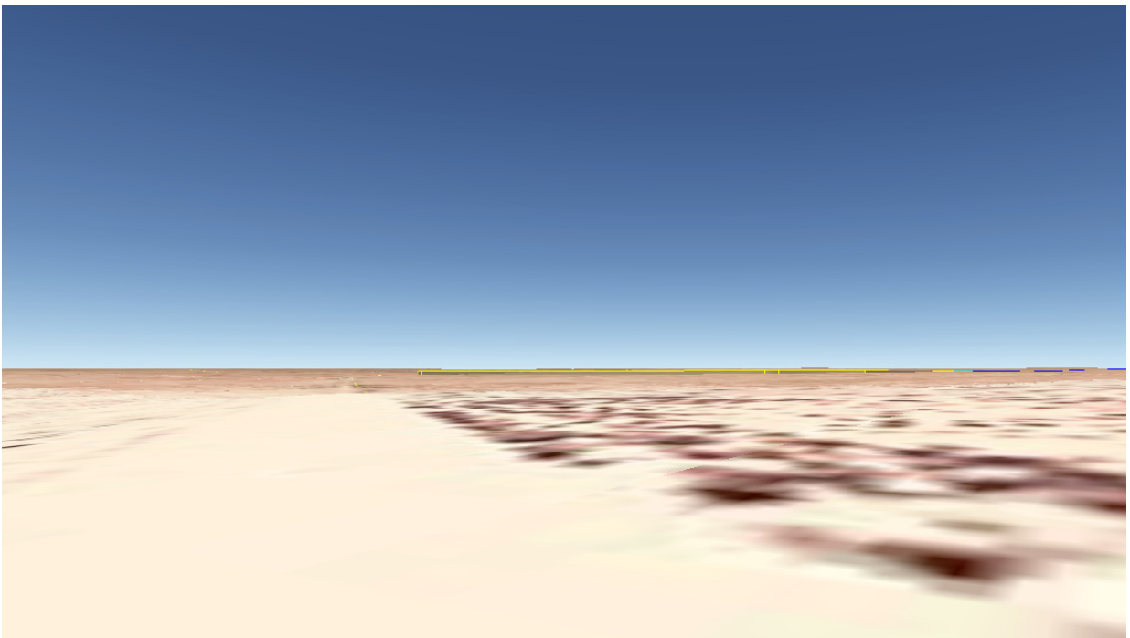
Figure 24: Google Earth 3D perspective view from similar northbound location (Yellow = Bravo PV, Green = Substation, Blue = Power Line).
