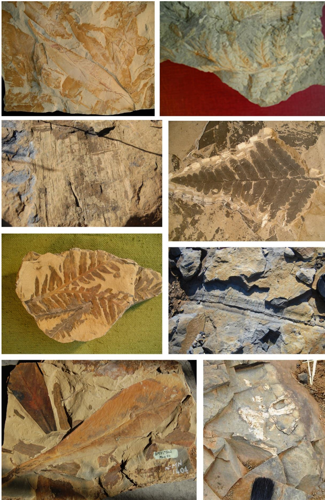
Figure 5: Selection of fossil plant impressions of the Glossopteris flora
