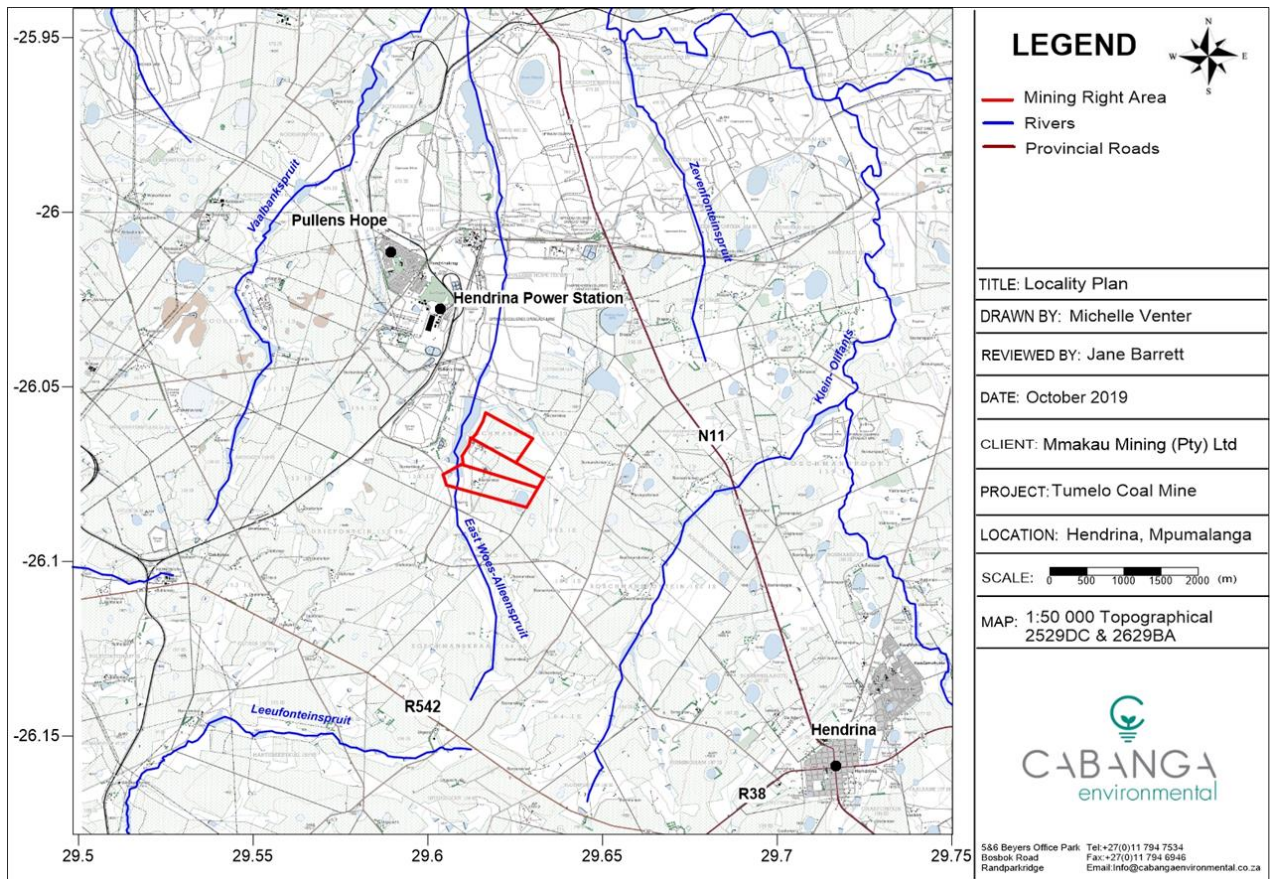
Figure 1: Site map, with the approved Mining Right Area (MRA) indicated in red. Map supplied by Cabanga Environmental
