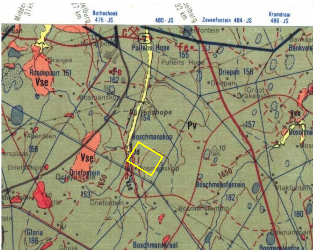
Figure 3: Geological map of the area between Hendrina Power Station and Hendrina town, for the existing MRA on Farm Boschmanskop 154 IS. The location of the project is indicated within the yellow rectangle. Abbreviations of the rock types are explained in Table 2. Map enlarged from the Geological Survey 1: 250 000 map 2628 East Rand.
