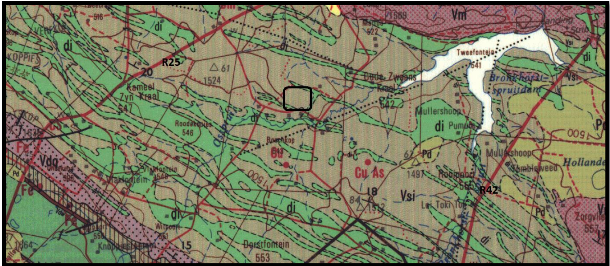
Figure 4: The geology of the development area.
