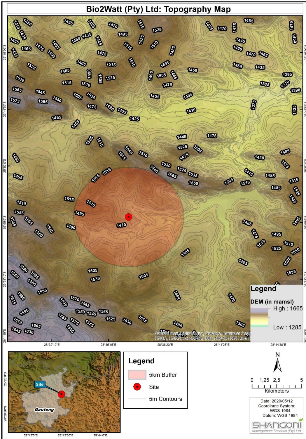
Figure 1: Topographic map of development (Shangoni).
