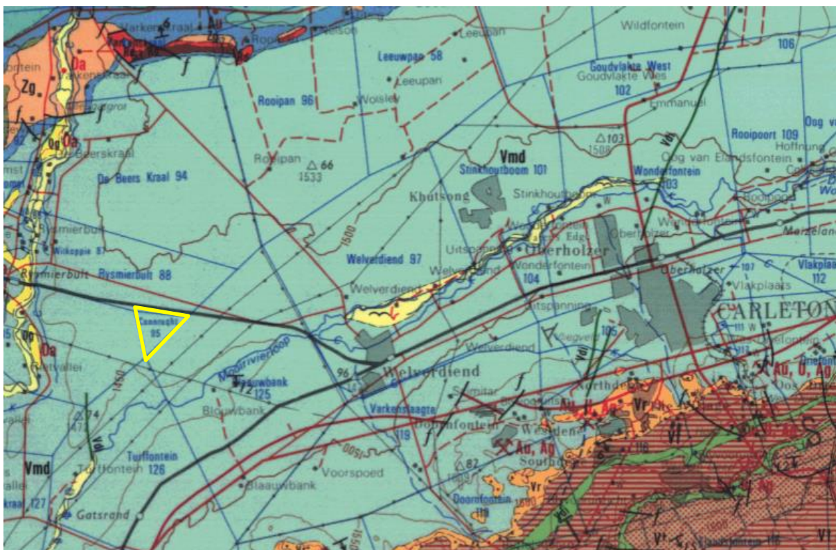
Figure 3: Geological map of the area around the Farm Douglasdale 95 IQ, west of Carltonville. Abbreviations of the rock types are explained in Table 2. Map enlarged from the Geological Survey 1: 250 000 map 2626 West Rand.
