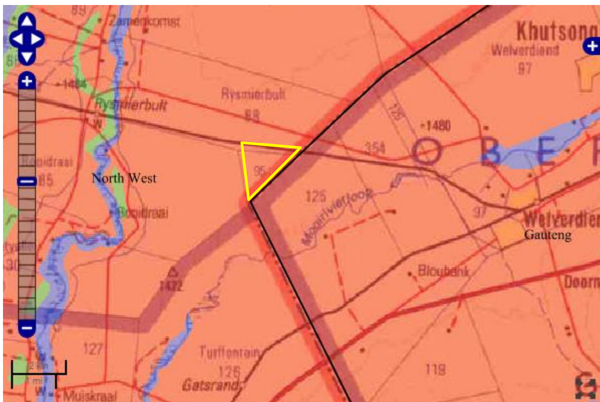
Figure 4: SAHRIS palaeosensitivity map for the site for the proposed Mopane PV 1 (yellow). Background colours indicate the following degrees of sensitivity: red = very highly sensitive; orange/yellow = high; green = moderate; blue = low; grey = insignificant/zero.
