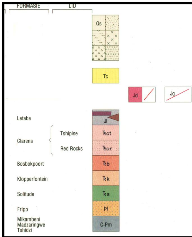
Figure 4: Northern Karoo Supergroup distribution and lithostratigraphy (Brandl and Pretorius 2000).
