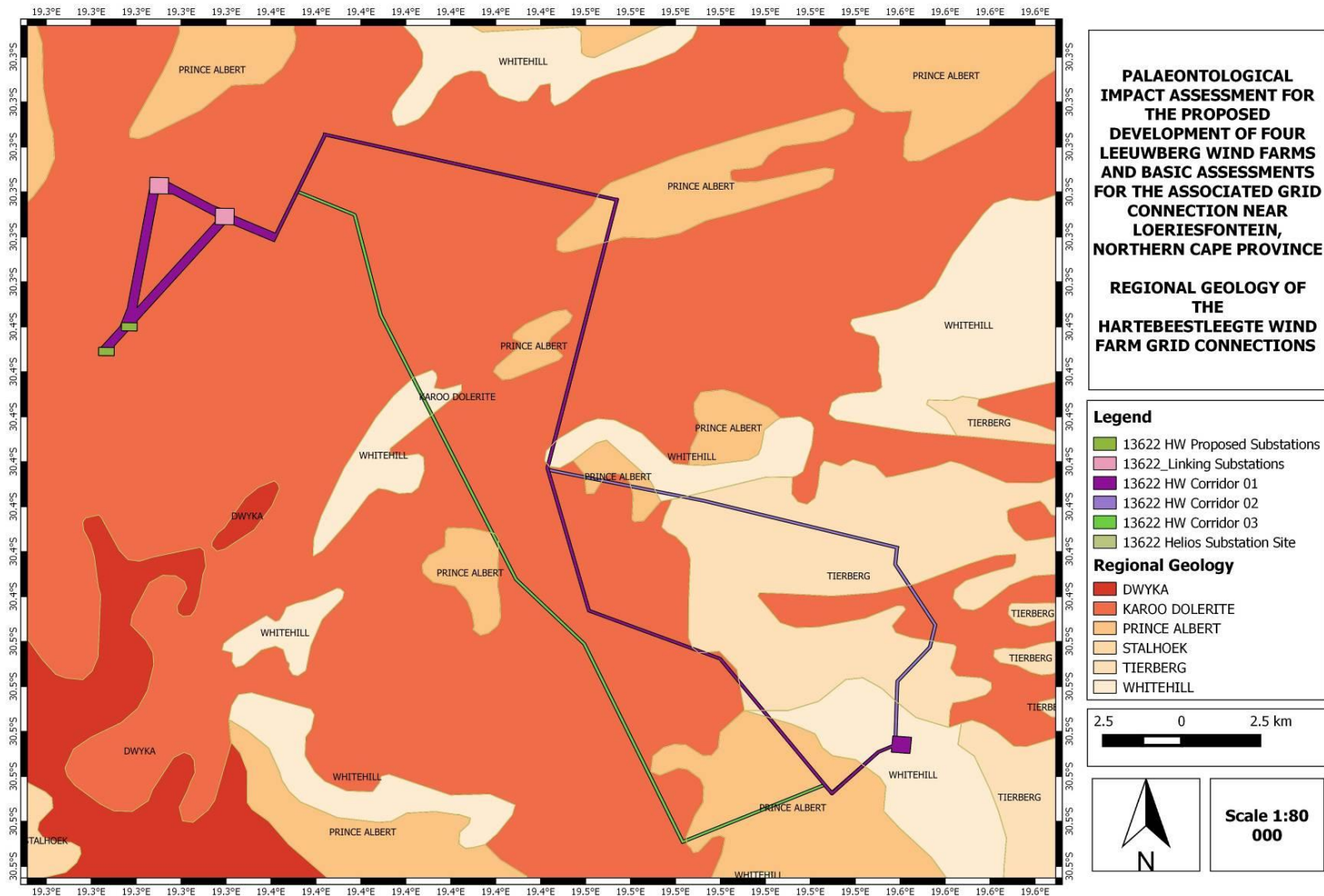
Figure 5: The surface geology of the proposed grid connection for the Hartbeest Leegte Wind Farm near Loeriesfontein in the Northern Cape Province. The development footprint is underlain by Karoo Dolerite as well as the Prince Albert, Whitehill and Tierberg Formations of the Ecca Group.
