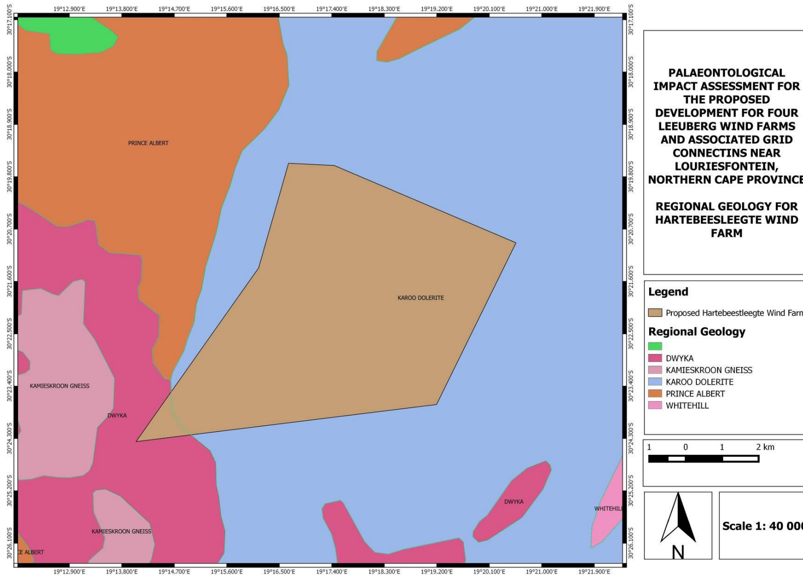
Figure 4: The surface geology of the proposed Hartebeest Leegte Wind Farm near Loeriesfontein in the Northern Cape Province. The development footprint is mostly underlain by Karoo Dolerite and a small area in the south west is underlain by the lowermost unit of the Karoo Supergroup, namely the Dwyka Group.
