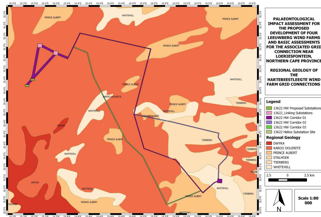
Figure 4: The surface geology of the proposed grid connection for the Hartebeest Leegte Wind Farm near Loeriesfontein in the Northern Cape Province. The development footprint is underlain by Karoo Dolerite as well as the Prince Albert, Whitehill and Tierberg Formations of the Ecca Group.
