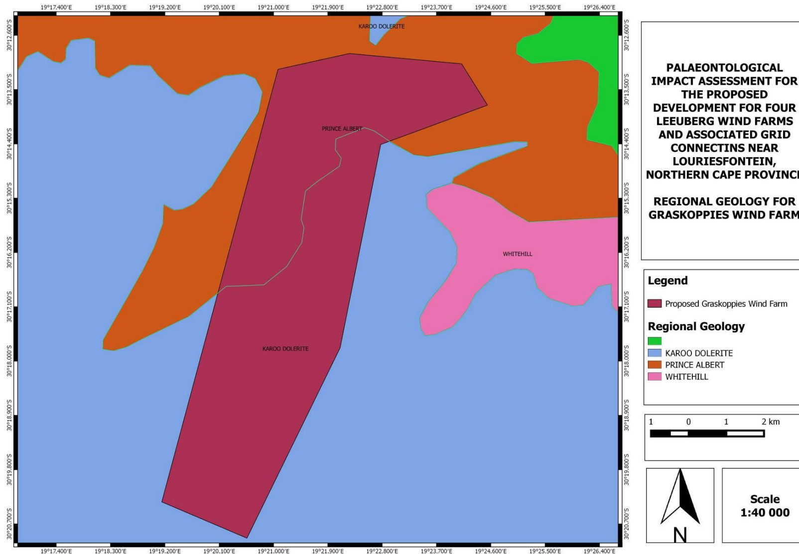
Figure 6: The surface geology of the proposed Graskoppies Wind Farm near Loriesfontein in the Northern Cape Province. The development footprint is underlain by Karoo Dolerite as well as the Prince Albert and Whitehill Formations of the Ecca Group.
