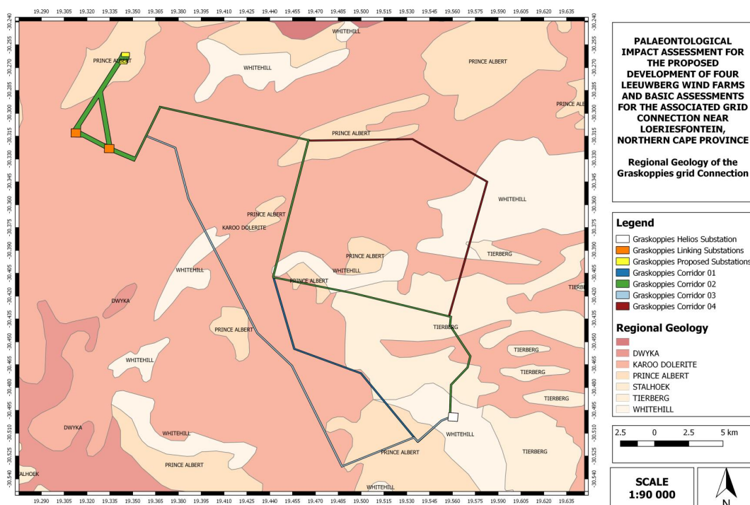
Figure 4: The surface geology of the proposed grid connection of Graskoppies Wind Farm near Loeriesfontein in the Northern Cape Province. The development footprint is underlain by Karoo Dolerite as well as the Prince Albert, Whitehill and Tierberg Formations of the Ecca Group.
