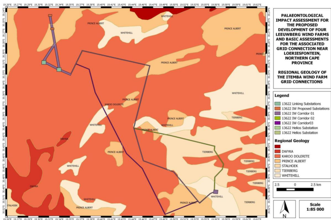
Figure 9: The surface geology of the proposed grid connection of the Itemba Wind Farm near Loeriesfontein in the Northern Cape Province. The development footprint is
